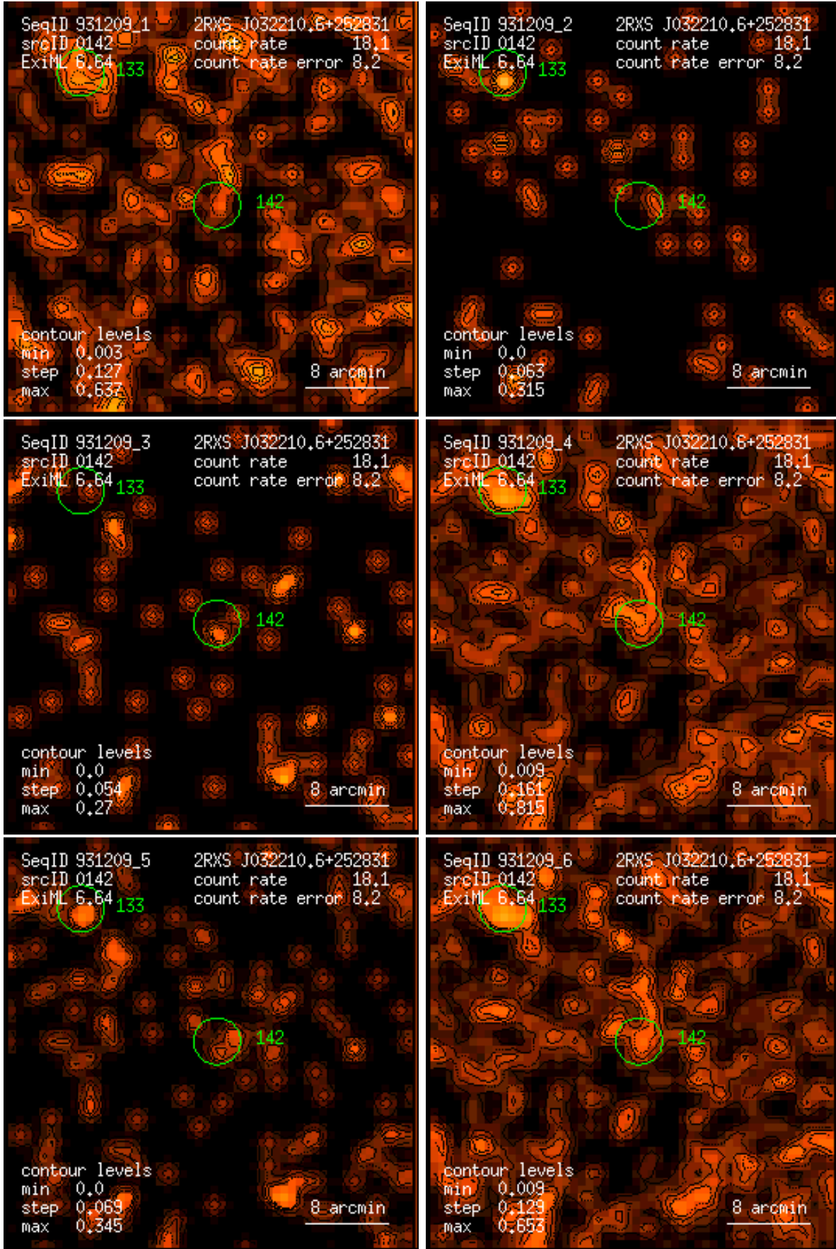
Figure 142: RASS 931209: detection 0142: band rate images, Gaussian filter: (1) PSPC channels 11 – 41, (2) 52 – 90, (3) 91 – 201, (4) 11 – 235, (5) 52 – 201, (6) 11 – 201. Broad band rates in counts/ks. Band rate contour levels in counts/ks/arcmin 2 .
