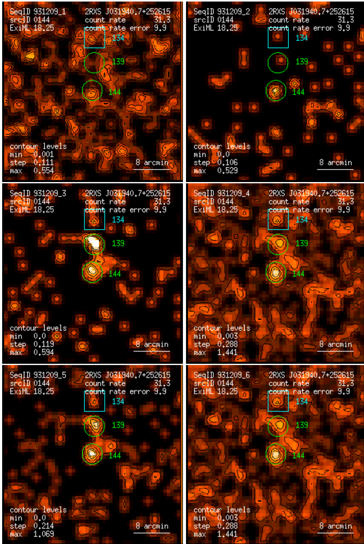
Figure 144: RASS 931209: detection 0144: band rate images, Gaussian filter: (1) PSPC channels 11 – 41, (2) 52 – 90, (3) 91 – 201, (4) 11 – 235, (5) 52 – 201, (6) 11 – 201. Broad band rates in counts/ks. Band rate contour levels in counts/ks/arcmin 2 .
