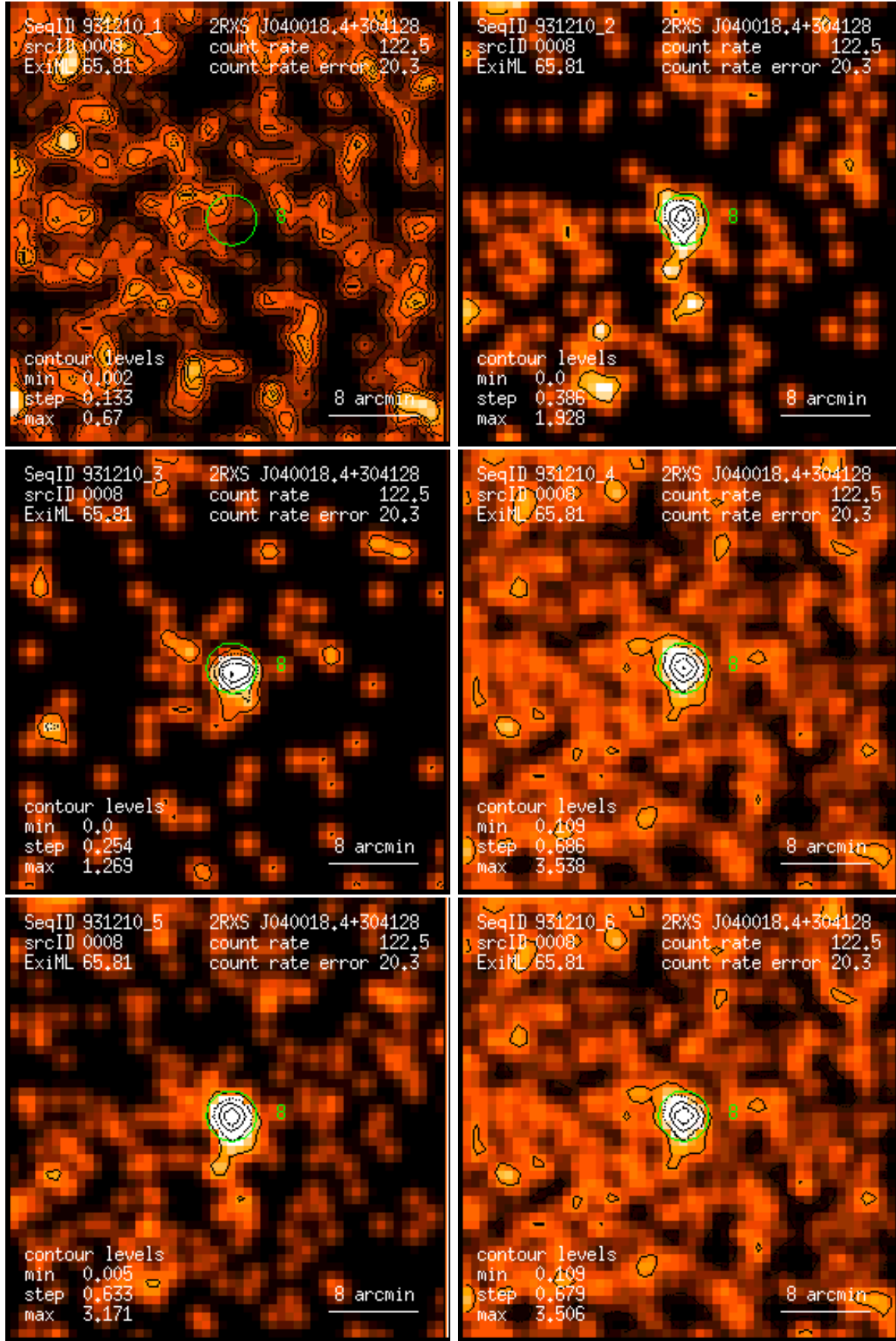
Figure 8: RASS 931210: detection 0008: band rate images, Gaussian filter: (1) PSPC channels 11 – 41, (2) 52 – 90, (3) 91 – 201, (4) 11 – 235, (5) 52 – 201, (6) 11 – 201. Broad band rates in counts/ks. Band rate contour levels in counts/ks/arcmin 2 .
