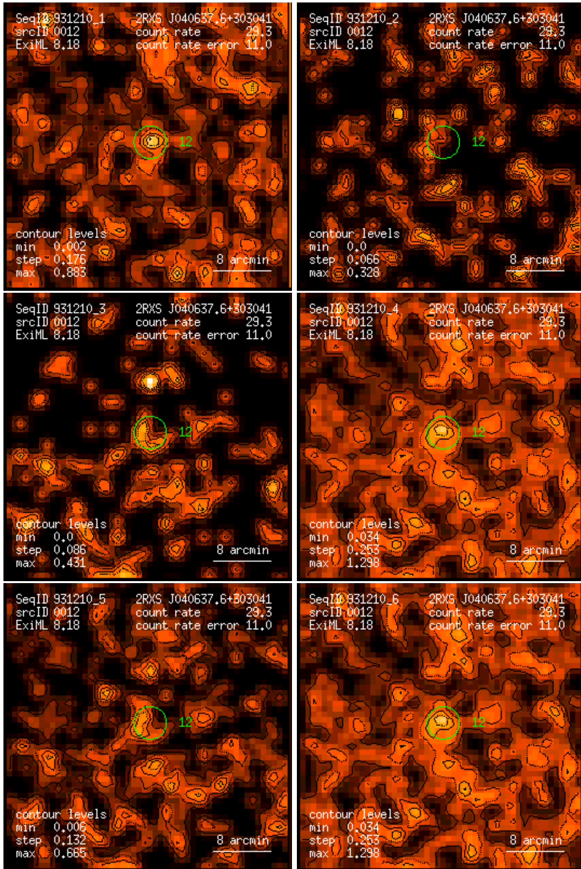
Figure 12: RASS 931210: detection 0012: band rate images, Gaussian filter: (1) PSPC channels 11 – 41, (2) 52 – 90, (3) 91 – 201, (4) 11 – 235, (5) 52 – 201, (6) 11 – 201. Broad band rates in counts/ks. Band rate contour levels in counts/ks/arcmin 2 .
