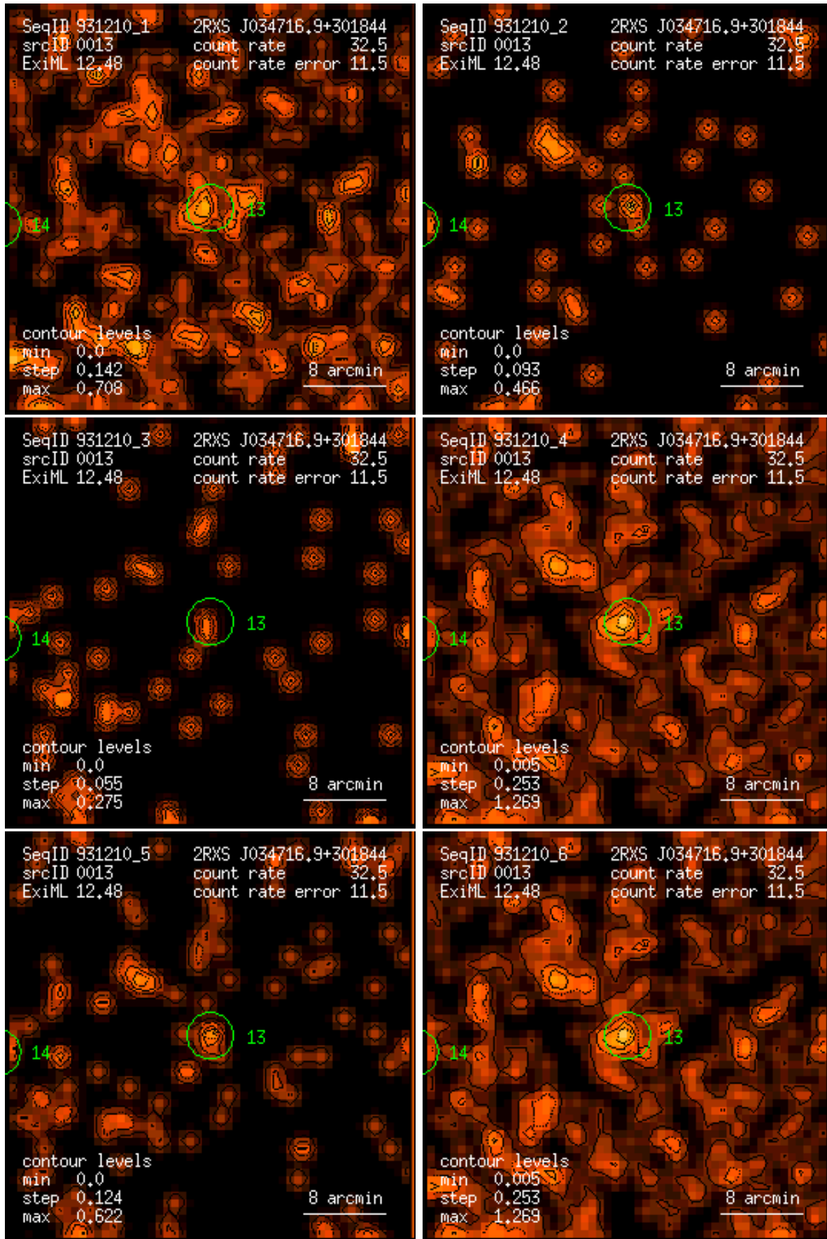
Figure 13: RASS 931210: detection 0013: band rate images, Gaussian filter: (1) PSPC channels 11 – 41, (2) 52 – 90, (3) 91 – 201, (4) 11 – 235, (5) 52 – 201, (6) 11 – 201. Broad band rates in counts/ks. Band rate contour levels in counts/ks/arcmin 2 .
