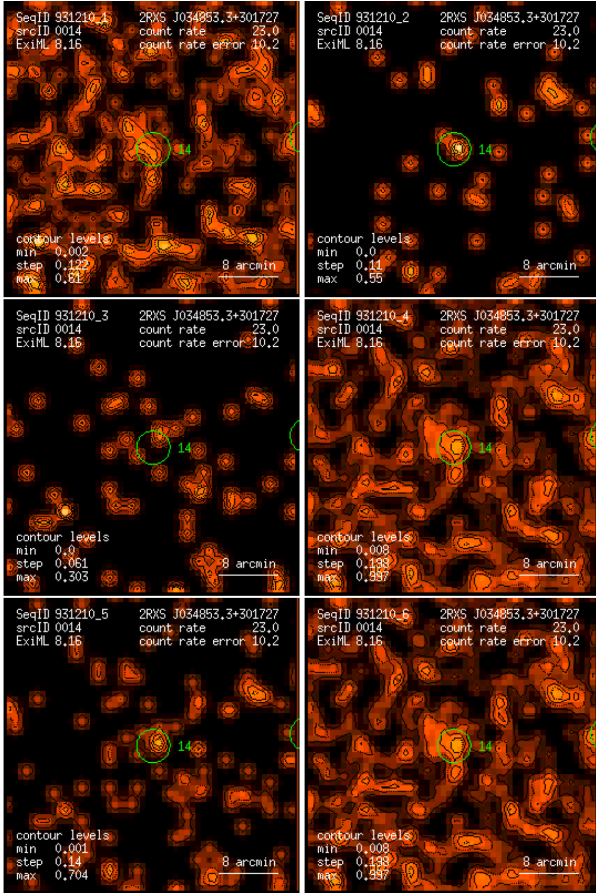
Figure 14: RASS 931210: detection 0014: band rate images, Gaussian filter: (1) PSPC channels 11 – 41, (2) 52 – 90, (3) 91 – 201, (4) 11 – 235, (5) 52 – 201, (6) 11 – 201. Broad band rates in counts/ks. Band rate contour levels in counts/ks/arcmin 2 .
