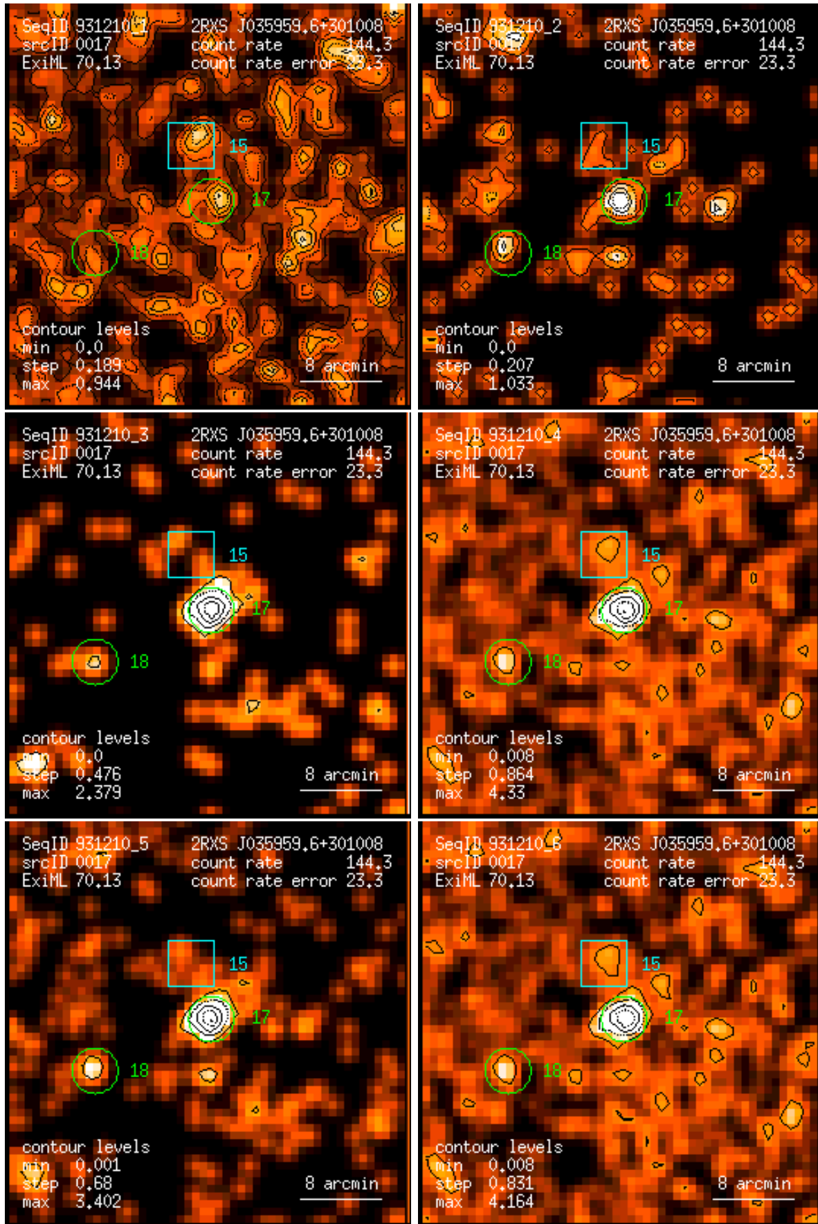
Figure 17: RASS 931210: detection 0017: band rate images, Gaussian filter: (1) PSPC channels 11 – 41, (2) 52 – 90, (3) 91 – 201, (4) 11 – 235, (5) 52 – 201, (6) 11 – 201. Broad band rates in counts/ks. Band rate contour levels in counts/ks/arcmin 2 .
