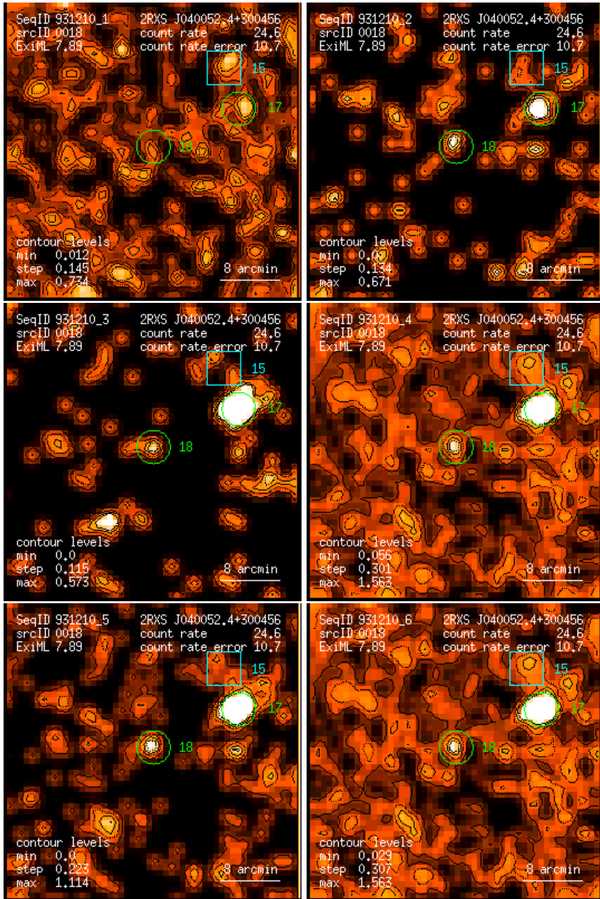
Figure 18: RASS 931210: detection 0018: band rate images, Gaussian filter: (1) PSPC channels 11 – 41, (2) 52 – 90, (3) 91 – 201, (4) 11 – 235, (5) 52 – 201, (6) 11 – 201. Broad band rates in counts/ks. Band rate contour levels in counts/ks/arcmin 2 .
