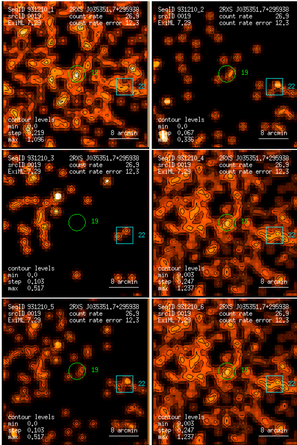
Figure 19: RASS 931210: detection 0019: band rate images, Gaussian filter: (1) PSPC channels 11 – 41, (2) 52 – 90, (3) 91 – 201, (4) 11 – 235, (5) 52 – 201, (6) 11 – 201. Broad band rates in counts/ks. Band rate contour levels in counts/ks/arcmin 2 .
