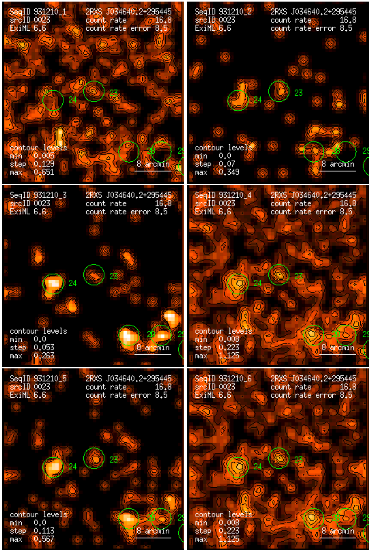
Figure 23: RASS 931210: detection 0023: band rate images, Gaussian filter: (1) PSPC channels 11 – 41, (2) 52 – 90, (3) 91 – 201, (4) 11 – 235, (5) 52 – 201, (6) 11 – 201. Broad band rates in counts/ks. Band rate contour levels in counts/ks/arcmin 2 .
