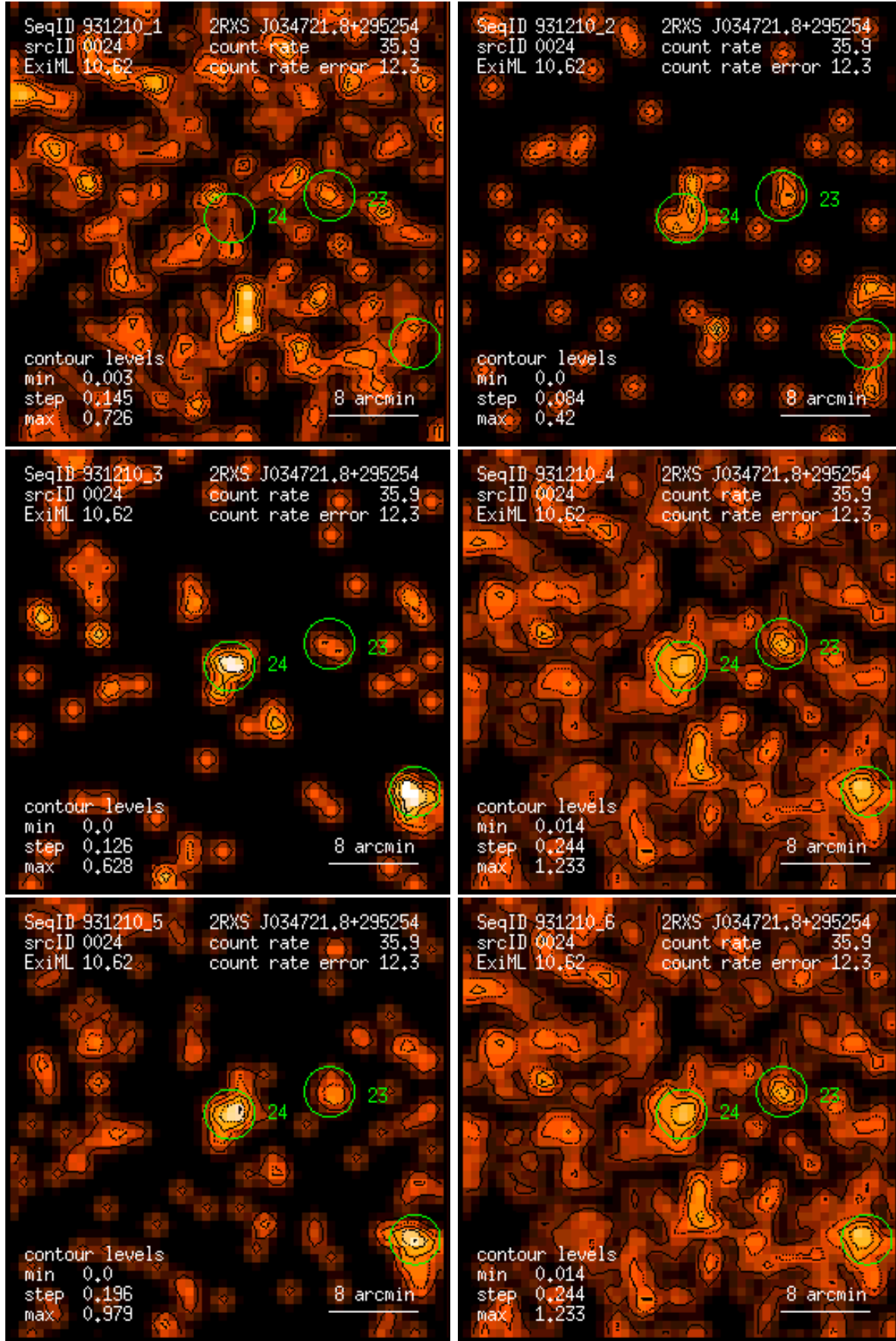
Figure 24: RASS 931210: detection 0024: band rate images, Gaussian filter: (1) PSPC channels 11 – 41, (2) 52 – 90, (3) 91 – 201, (4) 11 – 235, (5) 52 – 201, (6) 11 – 201. Broad band rates in counts/ks. Band rate contour levels in counts/ks/arcmin 2 .
