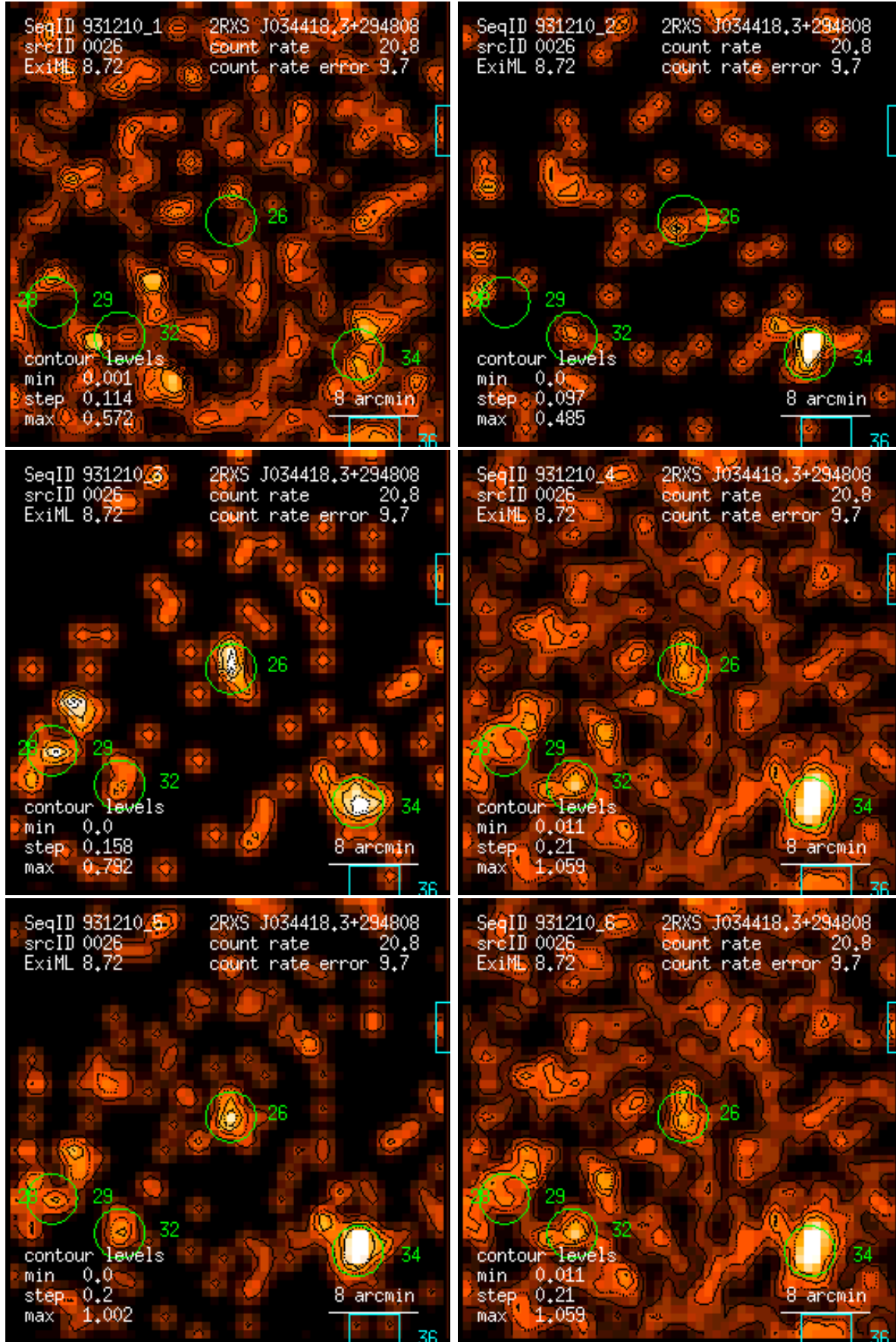
Figure 26: RASS 931210: detection 0026: band rate images, Gaussian filter: (1) PSPC channels 11 – 41, (2) 52 – 90, (3) 91 – 201, (4) 11 – 235, (5) 52 – 201, (6) 11 – 201. Broad band rates in counts/ks. Band rate contour levels in counts/ks/arcmin 2 .
