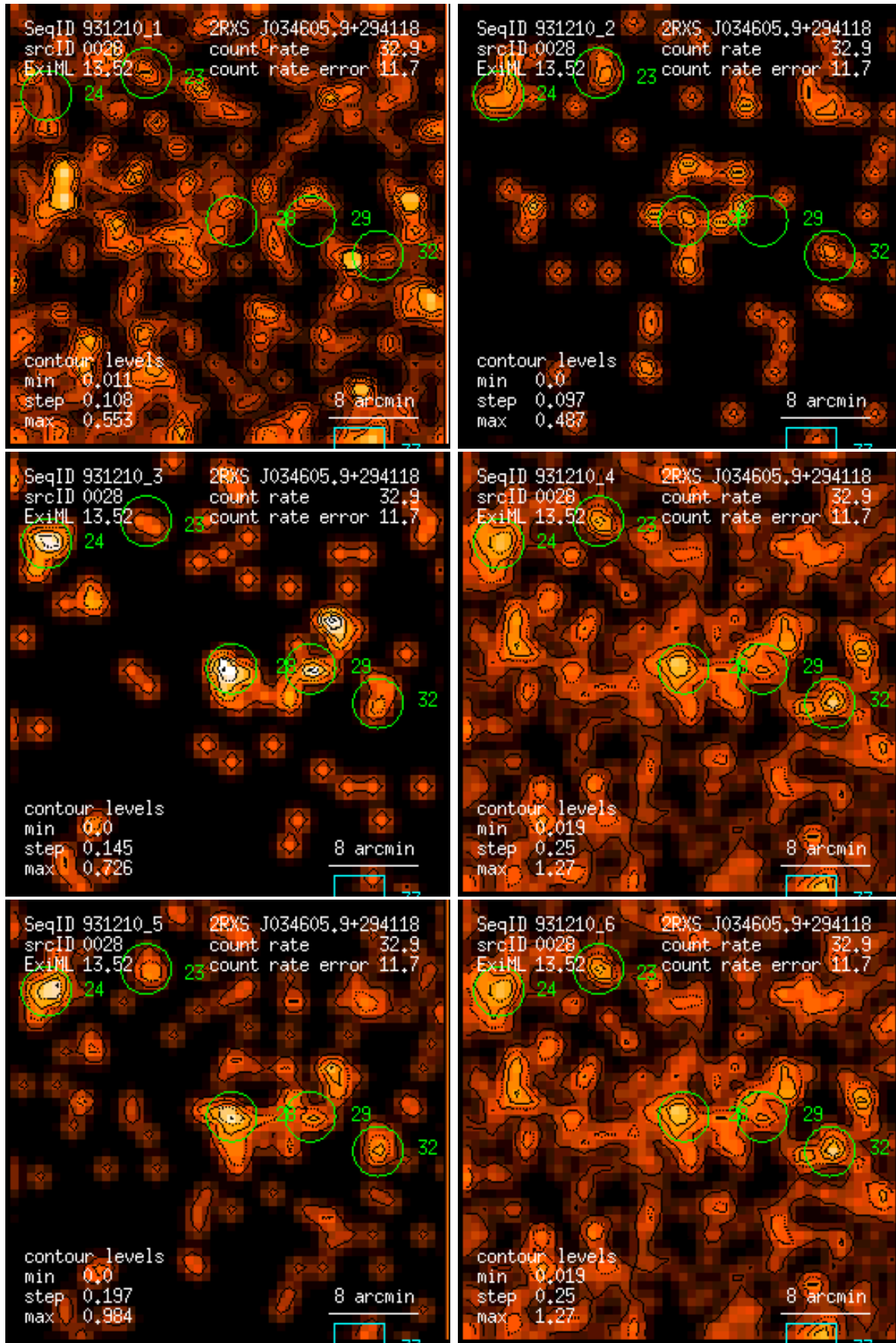
Figure 28: RASS 931210: detection 0028: band rate images, Gaussian filter: (1) PSPC channels 11 – 41, (2) 52 – 90, (3) 91 – 201, (4) 11 – 235, (5) 52 – 201, (6) 11 – 201. Broad band rates in counts/ks. Band rate contour levels in counts/ks/arcmin 2 .
