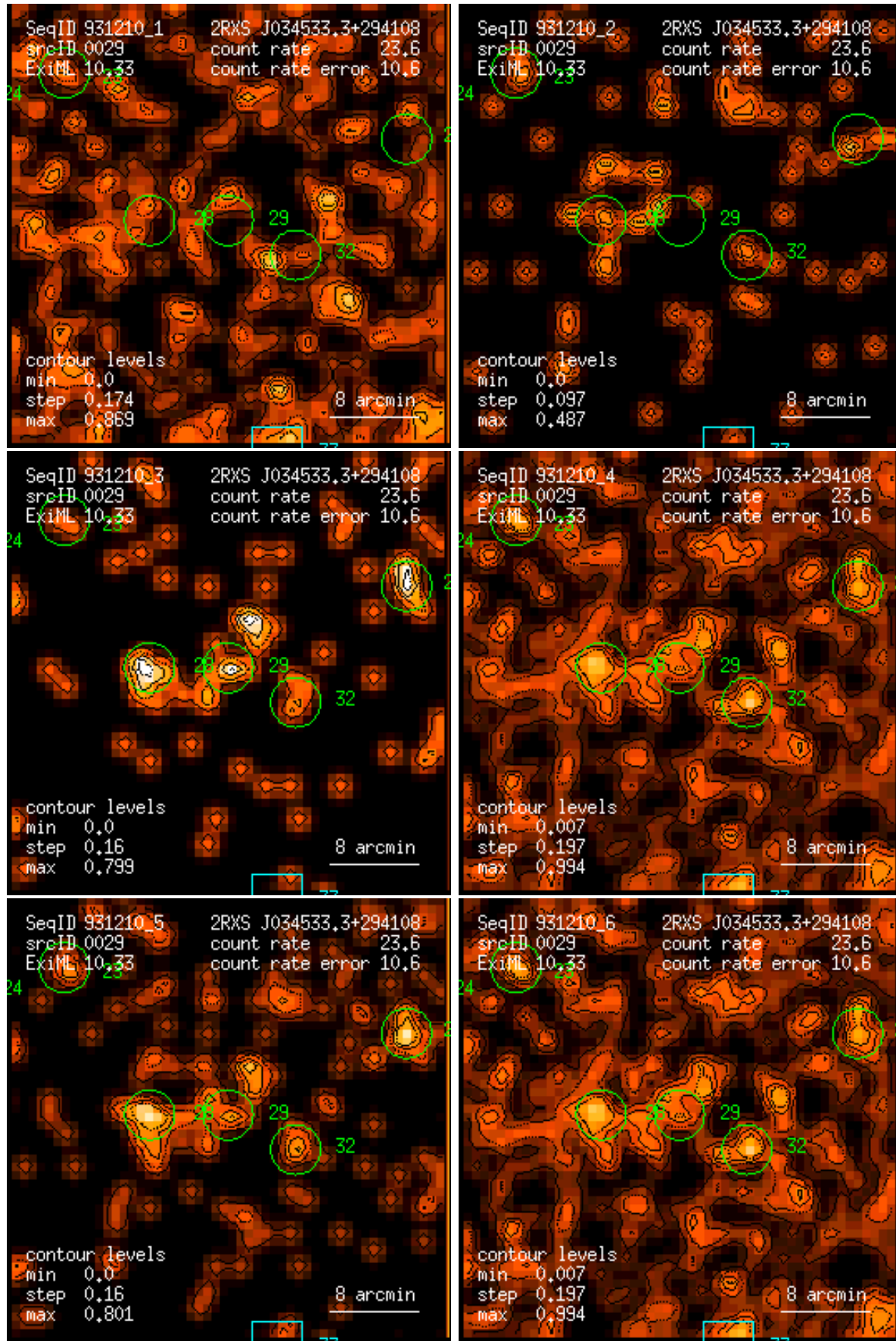
Figure 29: RASS 931210: detection 0029: band rate images, Gaussian filter: (1) PSPC channels 11 – 41, (2) 52 – 90, (3) 91 – 201, (4) 11 – 235, (5) 52 – 201, (6) 11 – 201. Broad band rates in counts/ks. Band rate contour levels in counts/ks/arcmin 2 .
