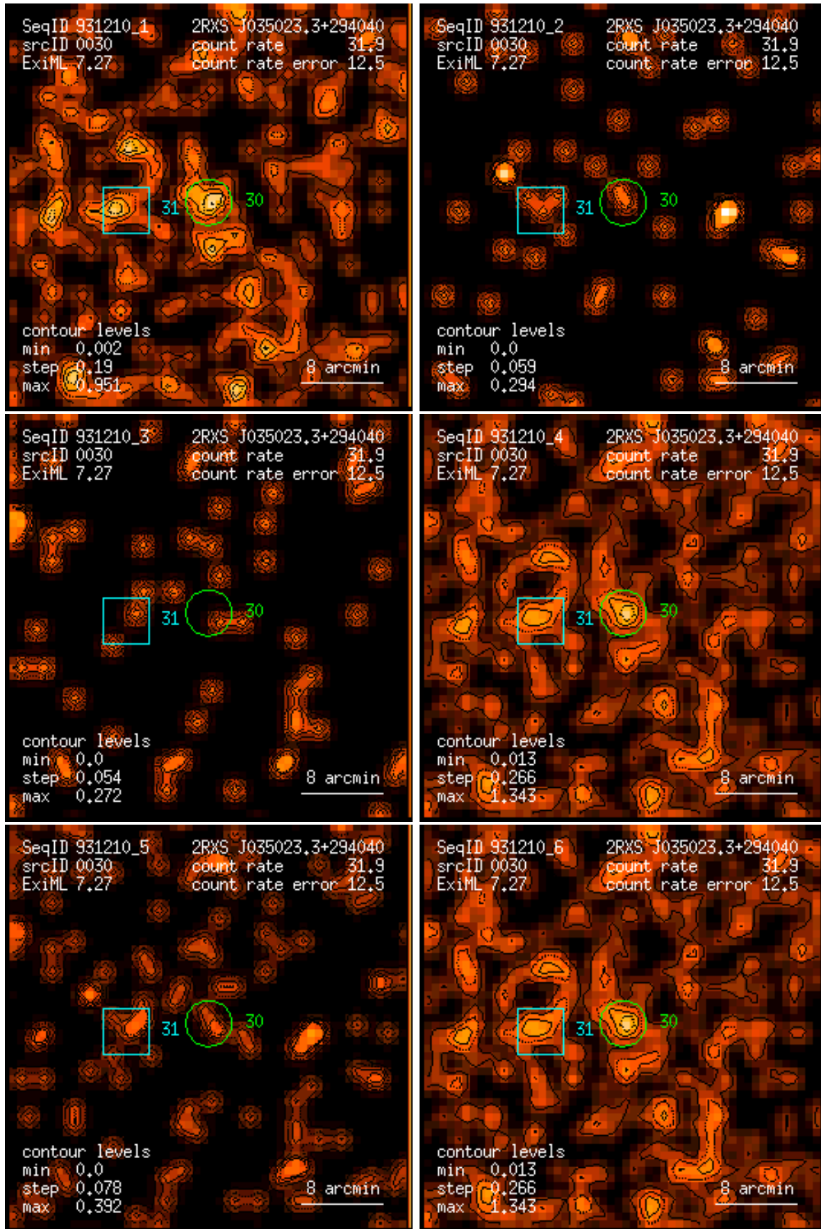
Figure 30: RASS 931210: detection 0030: band rate images, Gaussian filter: (1) PSPC channels 11 – 41, (2) 52 – 90, (3) 91 – 201, (4) 11 – 235, (5) 52 – 201, (6) 11 – 201. Broad band rates in counts/ks. Band rate contour levels in counts/ks/arcmin 2 .
