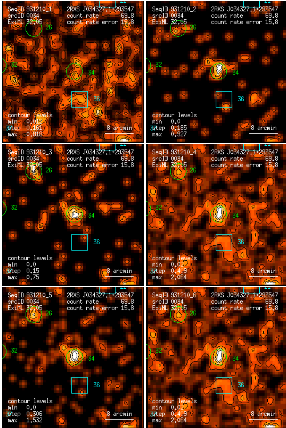
Figure 34: RASS 931210: detection 0034: band rate images, Gaussian filter: (1) PSPC channels 11 – 41, (2) 52 – 90, (3) 91 – 201, (4) 11 – 235, (5) 52 – 201, (6) 11 – 201. Broad band rates in counts/ks. Band rate contour levels in counts/ks/arcmin 2 .
