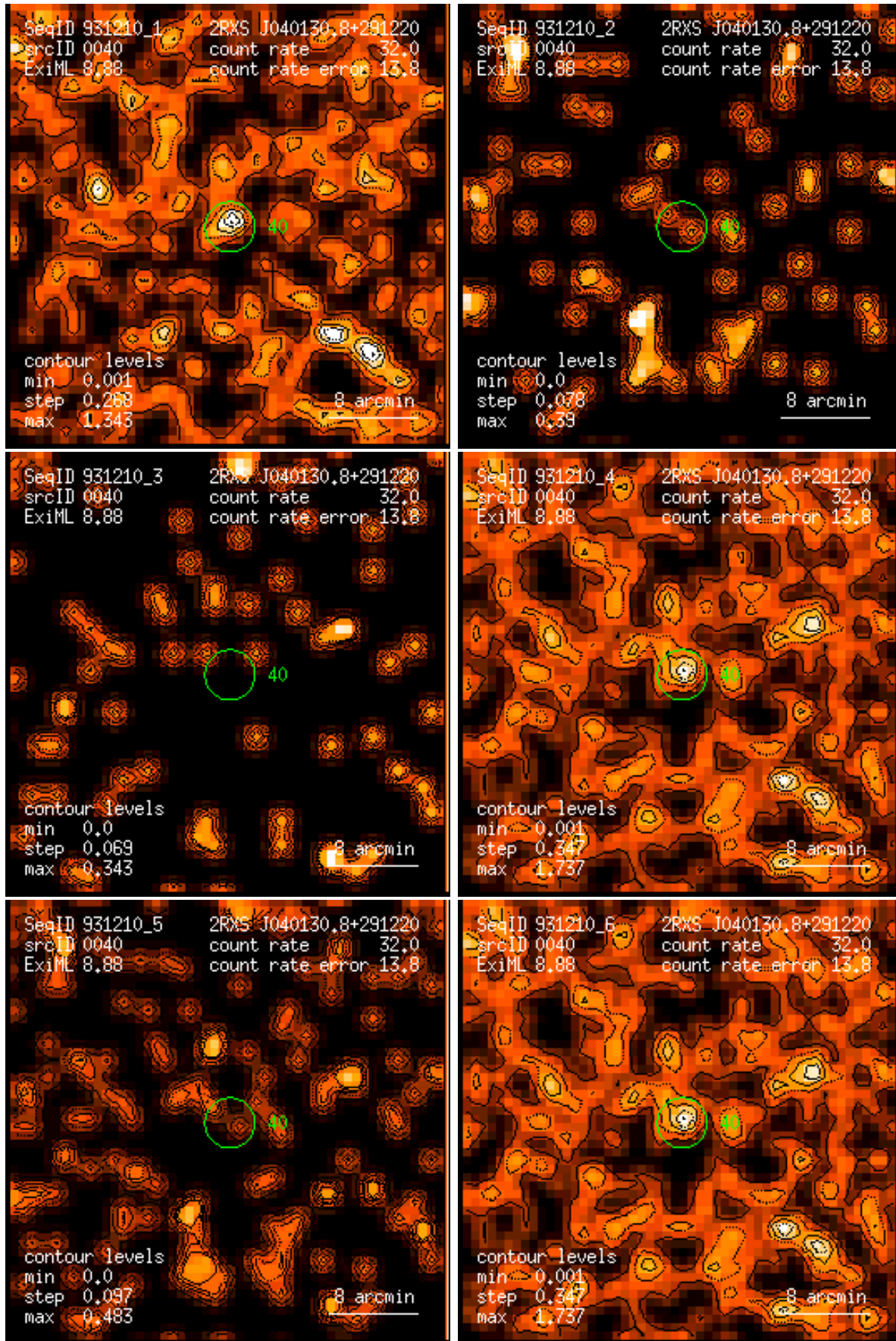
Figure 40: RASS 931210: detection 0040: band rate images, Gaussian filter: (1) PSPC channels 11 – 41, (2) 52 – 90, (3) 91 – 201, (4) 11 – 235, (5) 52 – 201, (6) 11 – 201. Broad band rates in counts/ks. Band rate contour levels in counts/ks/arcmin 2 .
