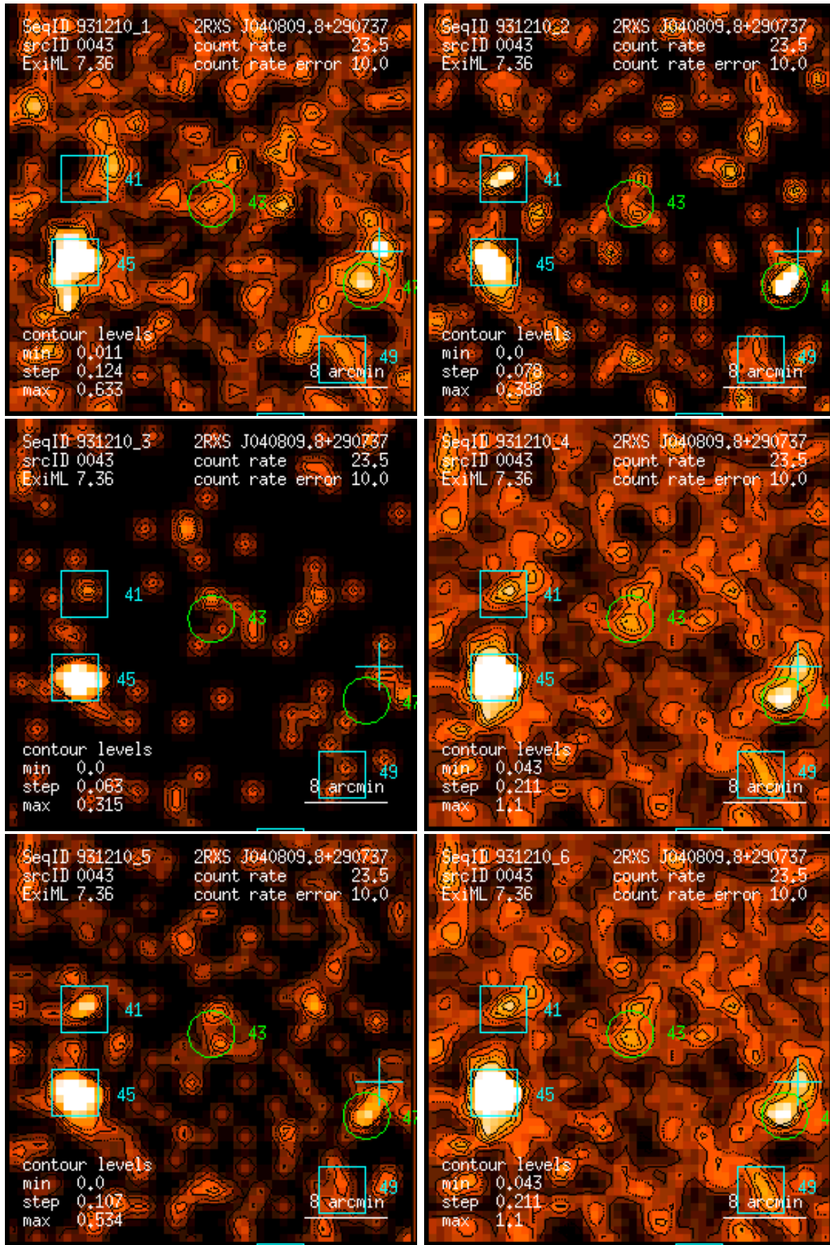
Figure 43: RASS 931210: detection 0043: band rate images, Gaussian filter: (1) PSPC channels 11 – 41, (2) 52 – 90, (3) 91 – 201, (4) 11 – 235, (5) 52 – 201, (6) 11 – 201. Broad band rates in counts/ks. Band rate contour levels in counts/ks/arcmin 2 .
