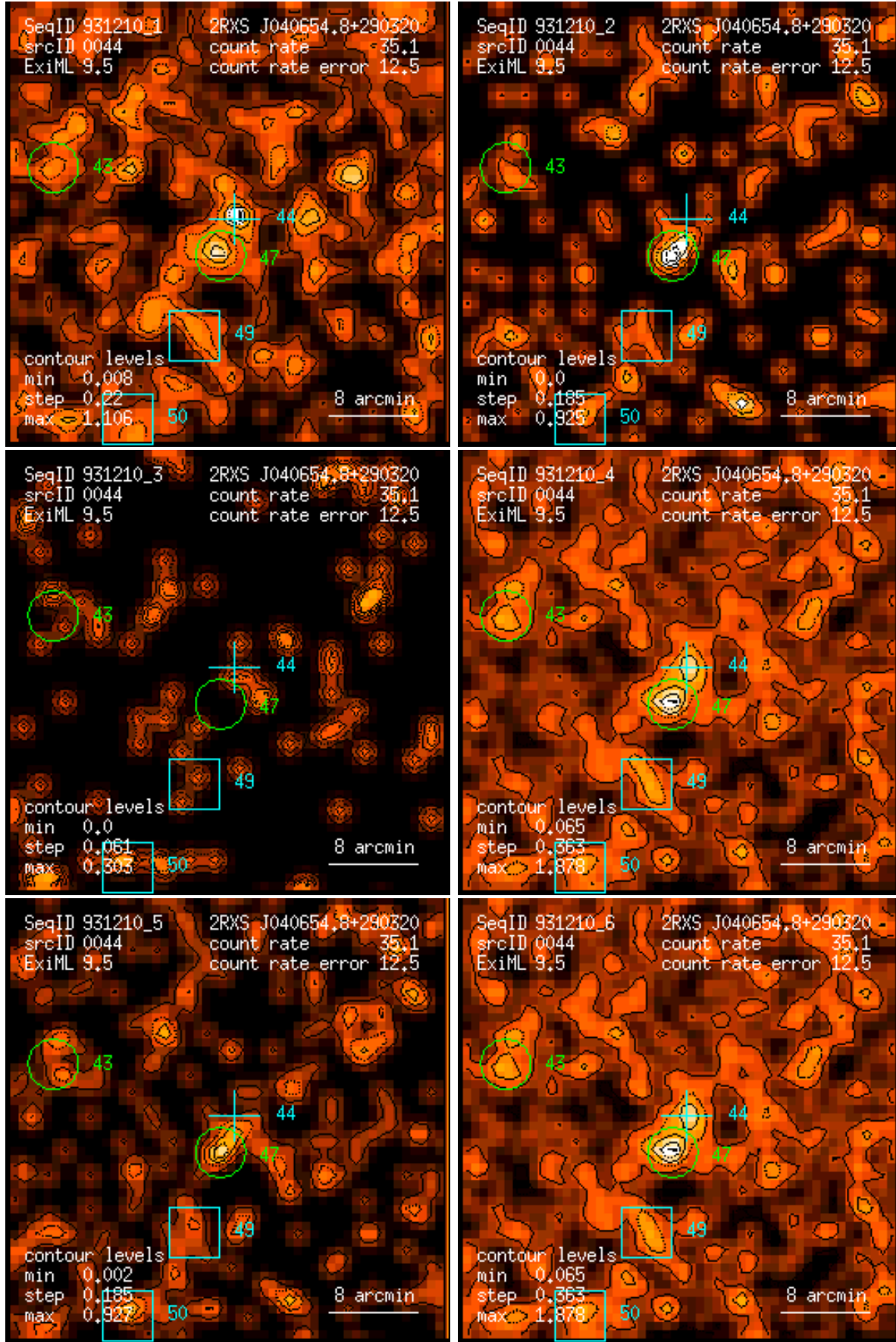
Figure 44: RASS 931210: detection 0044: band rate images, Gaussian filter: (1) PSPC channels 11 – 41, (2) 52 – 90, (3) 91 – 201, (4) 11 – 235, (5) 52 – 201, (6) 11 – 201. Broad band rates in counts/ks. Band rate contour levels in counts/ks/arcmin 2 .
