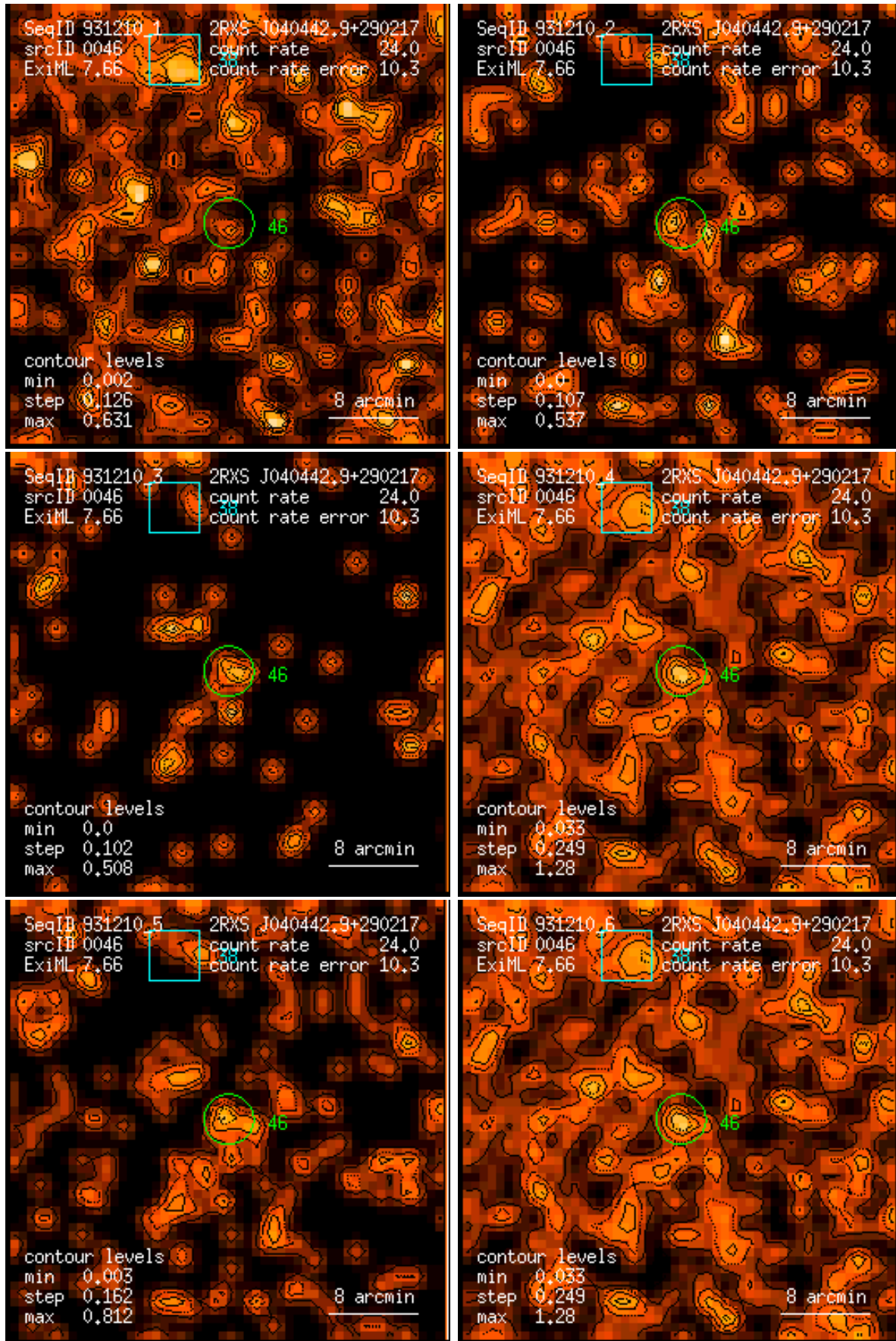
Figure 46: RASS 931210: detection 0046: band rate images, Gaussian filter: (1) PSPC channels 11 – 41, (2) 52 – 90, (3) 91 – 201, (4) 11 – 235, (5) 52 – 201, (6) 11 – 201. Broad band rates in counts/ks. Band rate contour levels in counts/ks/arcmin 2 .
