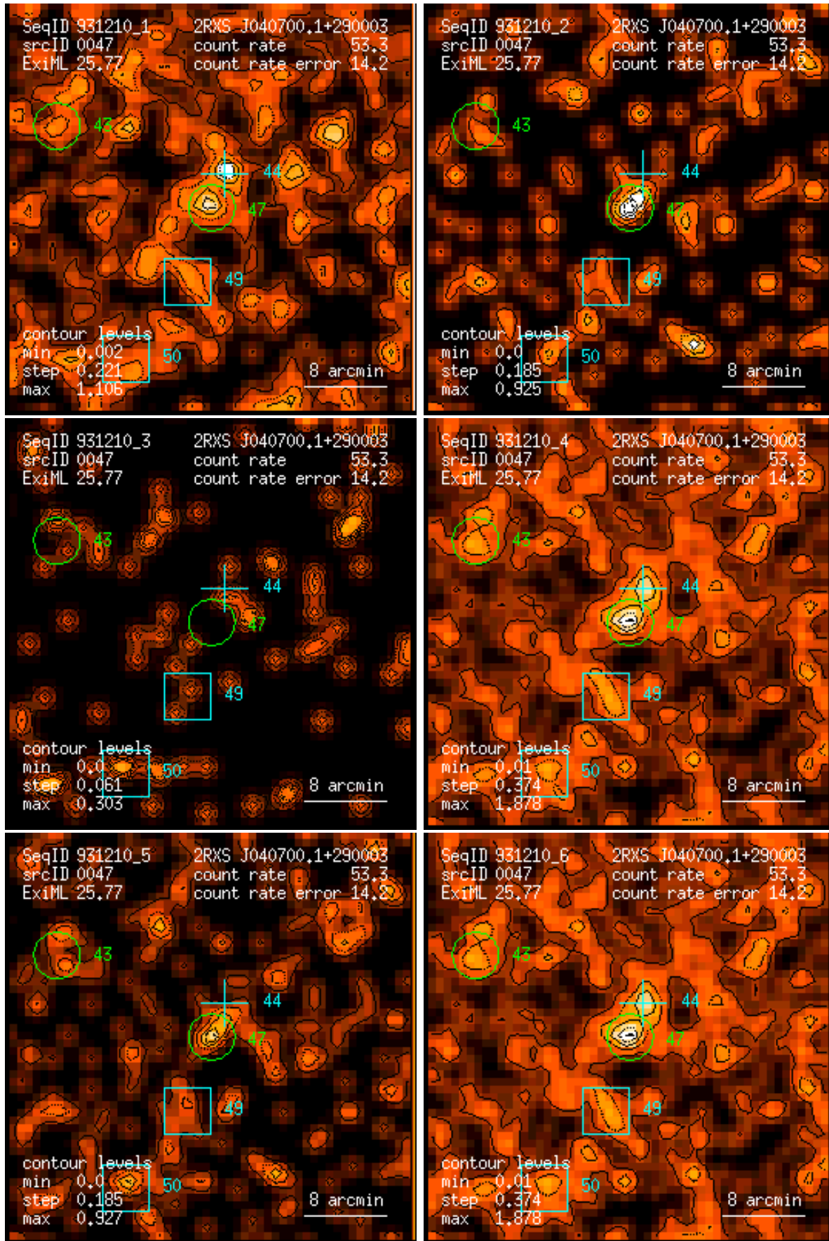
Figure 47: RASS 931210: detection 0047: band rate images, Gaussian filter: (1) PSPC channels 11 – 41, (2) 52 – 90, (3) 91 – 201, (4) 11 – 235, (5) 52 – 201, (6) 11 – 201. Broad band rates in counts/ks. Band rate contour levels in counts/ks/arcmin 2 .
