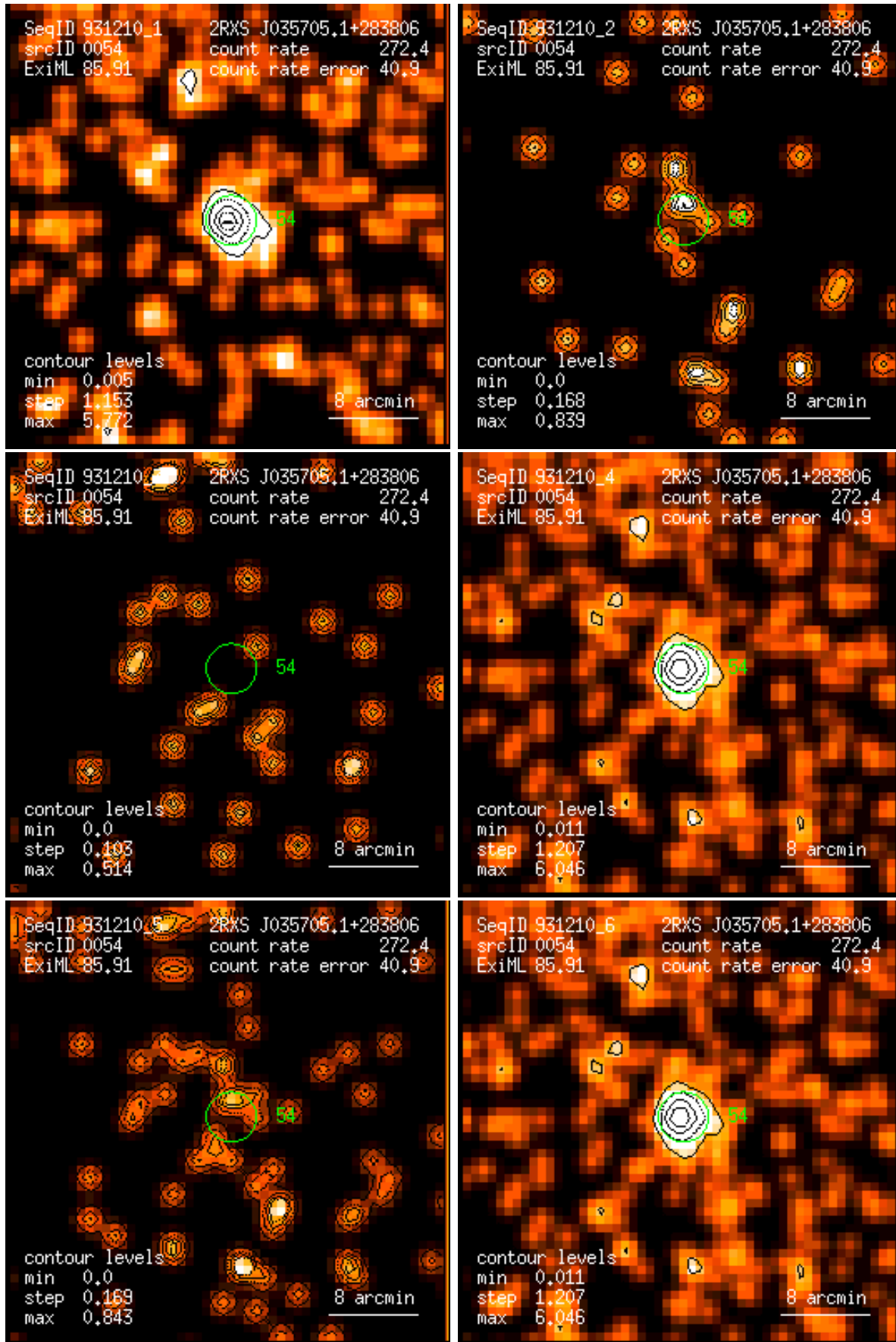
Figure 54: RASS 931210: detection 0054: band rate images, Gaussian filter: (1) PSPC channels 11 – 41, (2) 52 – 90, (3) 91 – 201, (4) 11 – 235, (5) 52 – 201, (6) 11 – 201. Broad band rates in counts/ks. Band rate contour levels in counts/ks/arcmin 2 .
