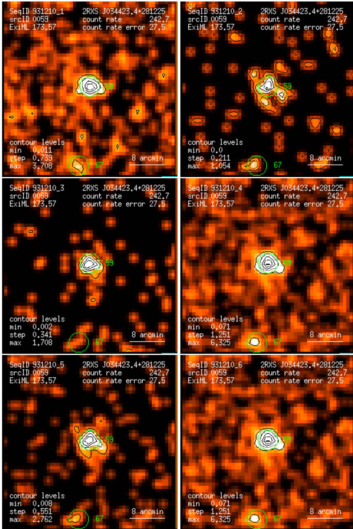
Figure 59: RASS 931210: detection 0059: band rate images, Gaussian filter: (1) PSPC channels 11 – 41, (2) 52 – 90, (3) 91 – 201, (4) 11 – 235, (5) 52 – 201, (6) 11 – 201. Broad band rates in counts/ks. Band rate contour levels in counts/ks/arcmin 2 .
