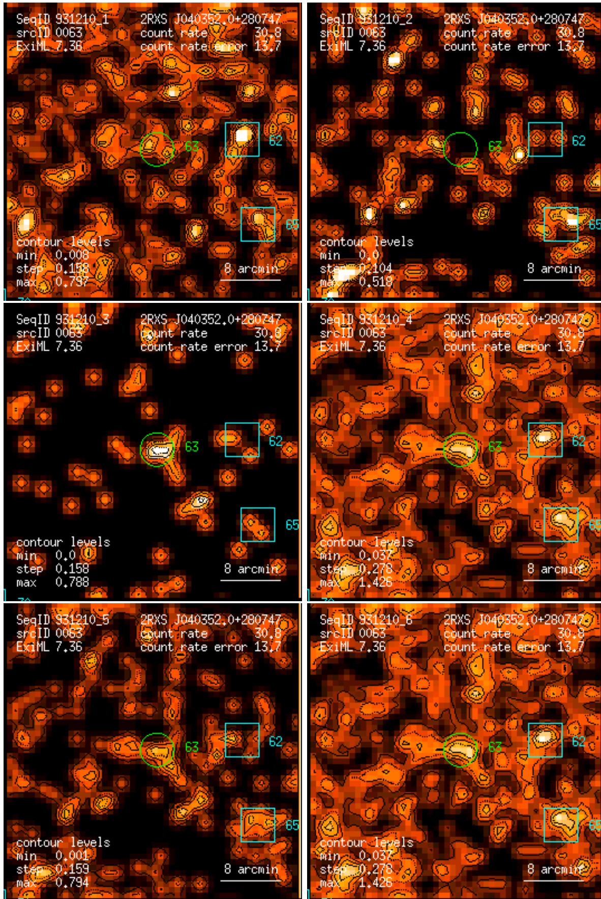
Figure 63: RASS 931210: detection 0063: band rate images, Gaussian filter: (1) PSPC channels 11 – 41, (2) 52 – 90, (3) 91 – 201, (4) 11 – 235, (5) 52 – 201, (6) 11 – 201. Broad band rates in counts/ks. Band rate contour levels in counts/ks/arcmin 2 .
