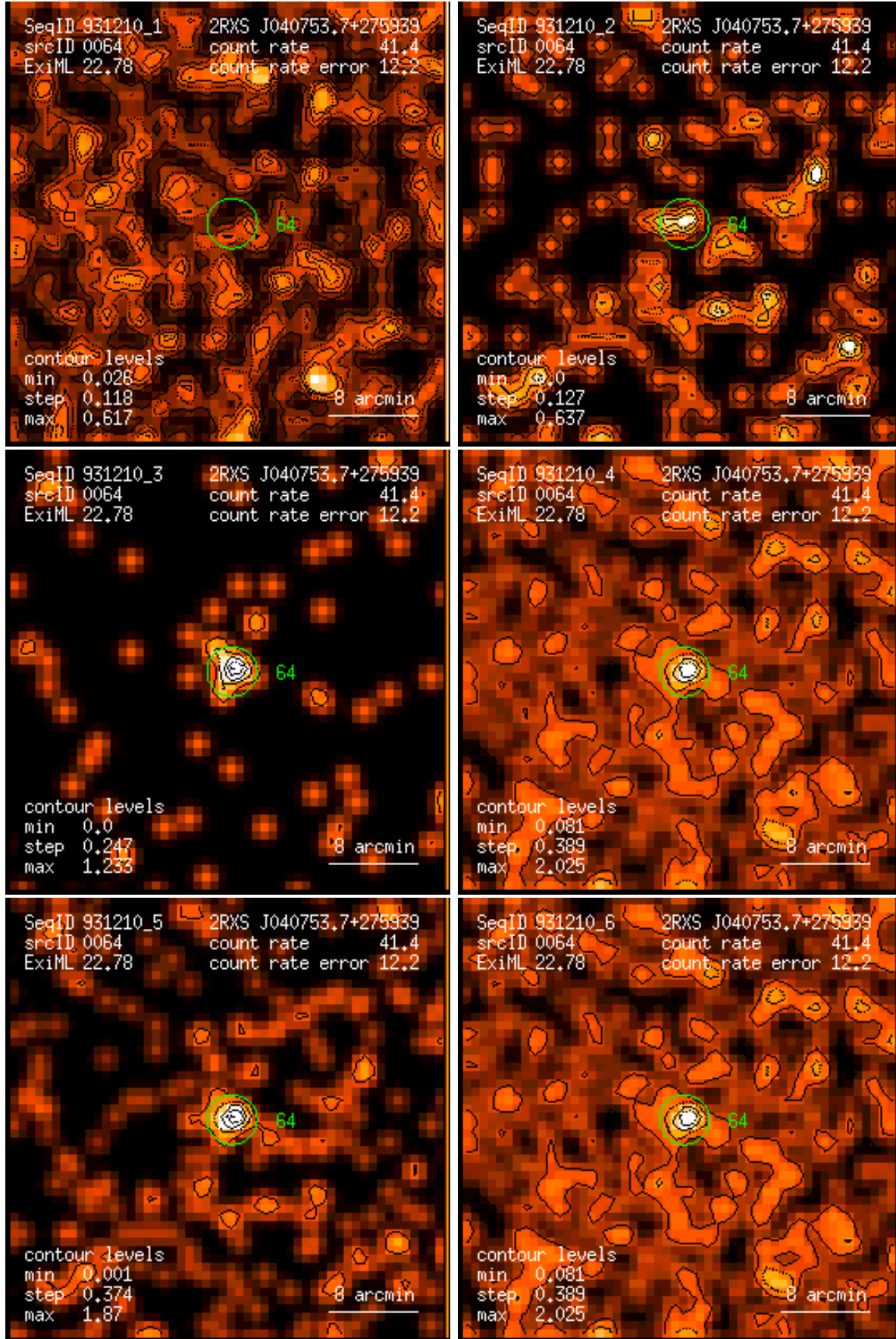
Figure 64: RASS 931210: detection 0064: band rate images, Gaussian filter: (1) PSPC channels 11 – 41, (2) 52 – 90, (3) 91 – 201, (4) 11 – 235, (5) 52 – 201, (6) 11 – 201. Broad band rates in counts/ks. Band rate contour levels in counts/ks/arcmin 2 .
