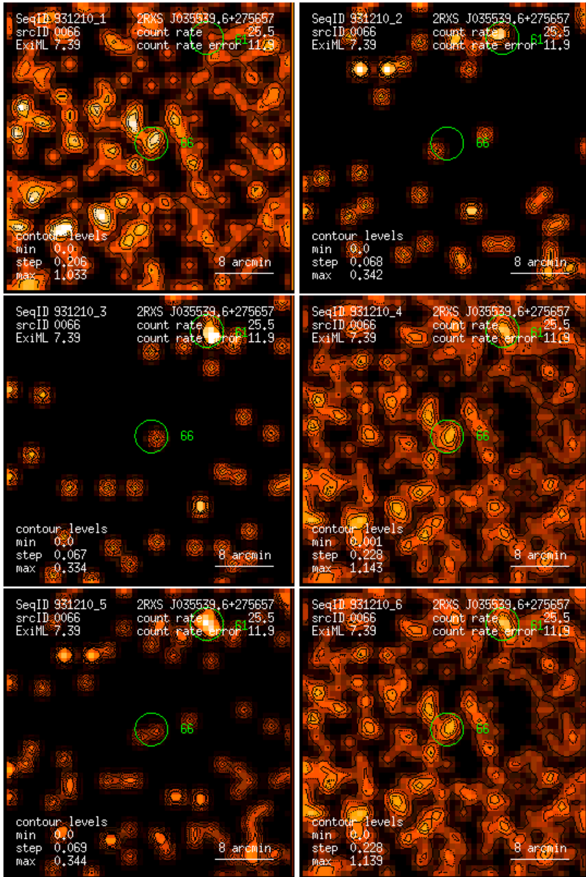
Figure 66: RASS 931210: detection 0066: band rate images, Gaussian filter: (1) PSPC channels 11 – 41, (2) 52 – 90, (3) 91 – 201, (4) 11 – 235, (5) 52 – 201, (6) 11 – 201. Broad band rates in counts/ks. Band rate contour levels in counts/ks/arcmin 2 .
