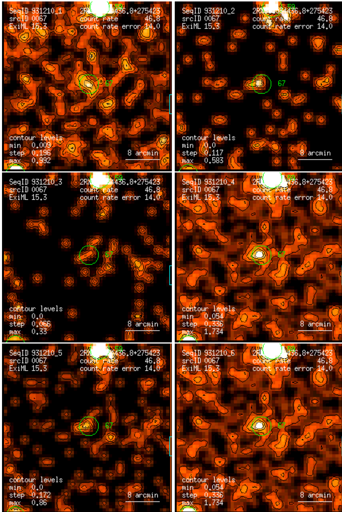
Figure 67: RASS 931210: detection 0067: band rate images, Gaussian filter: (1) PSPC channels 11 – 41, (2) 52 – 90, (3) 91 – 201, (4) 11 – 235, (5) 52 – 201, (6) 11 – 201. Broad band rates in counts/ks. Band rate contour levels in counts/ks/arcmin 2 .
