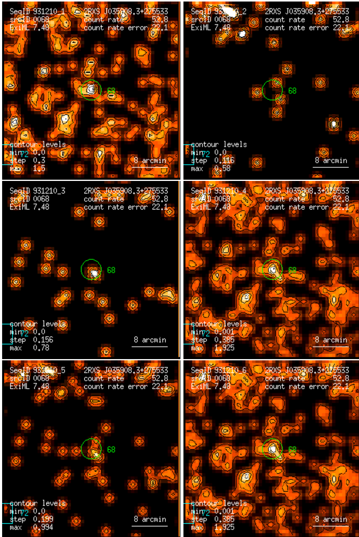
Figure 68: RASS 931210: detection 0068: band rate images, Gaussian filter: (1) PSPC channels 11 – 41, (2) 52 – 90, (3) 91 – 201, (4) 11 – 235, (5) 52 – 201, (6) 11 – 201. Broad band rates in counts/ks. Band rate contour levels in counts/ks/arcmin 2 .
