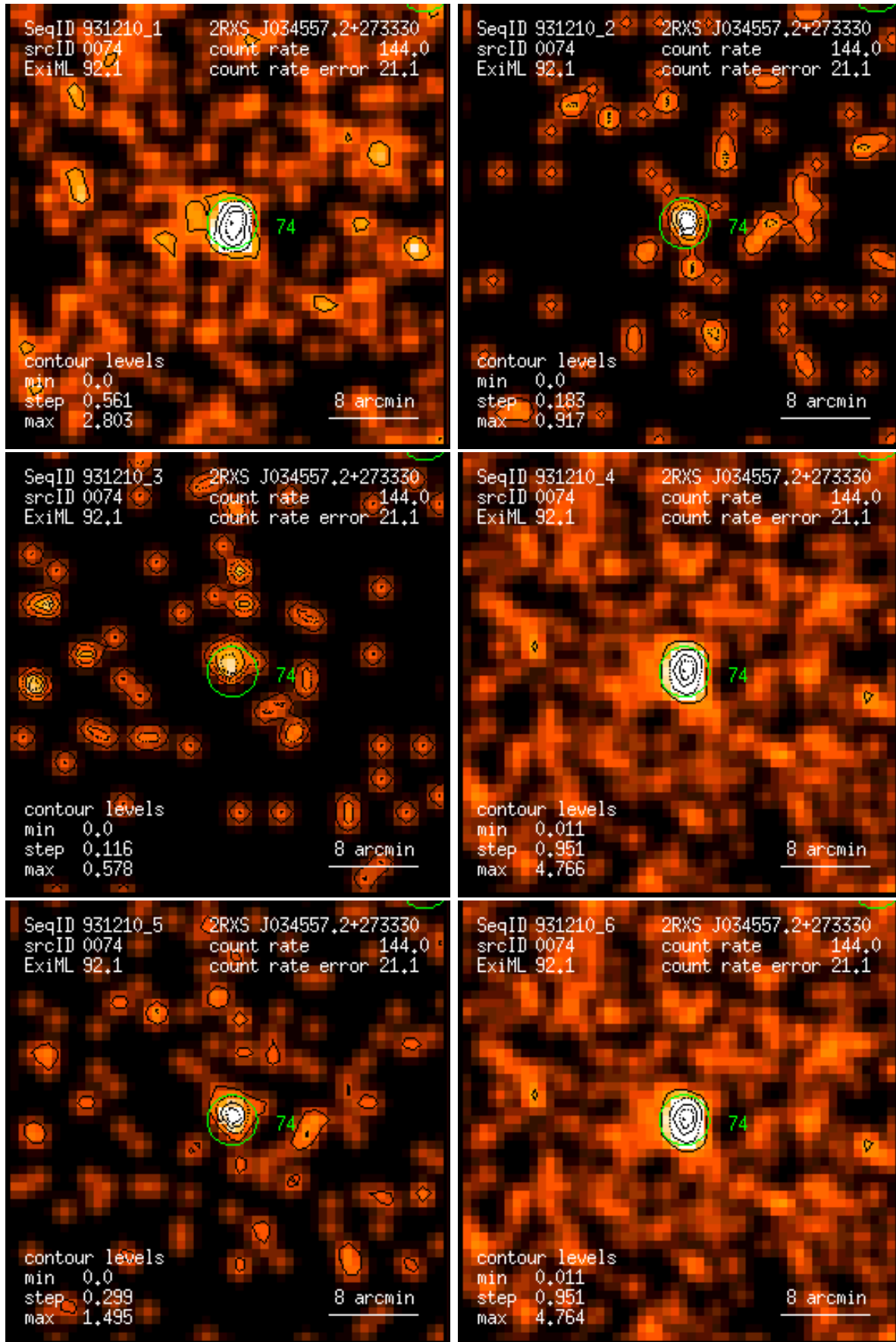
Figure 74: RASS 931210: detection 0074: band rate images, Gaussian filter: (1) PSPC channels 11 – 41, (2) 52 – 90, (3) 91 – 201, (4) 11 – 235, (5) 52 – 201, (6) 11 – 201. Broad band rates in counts/ks. Band rate contour levels in counts/ks/arcmin 2 .
