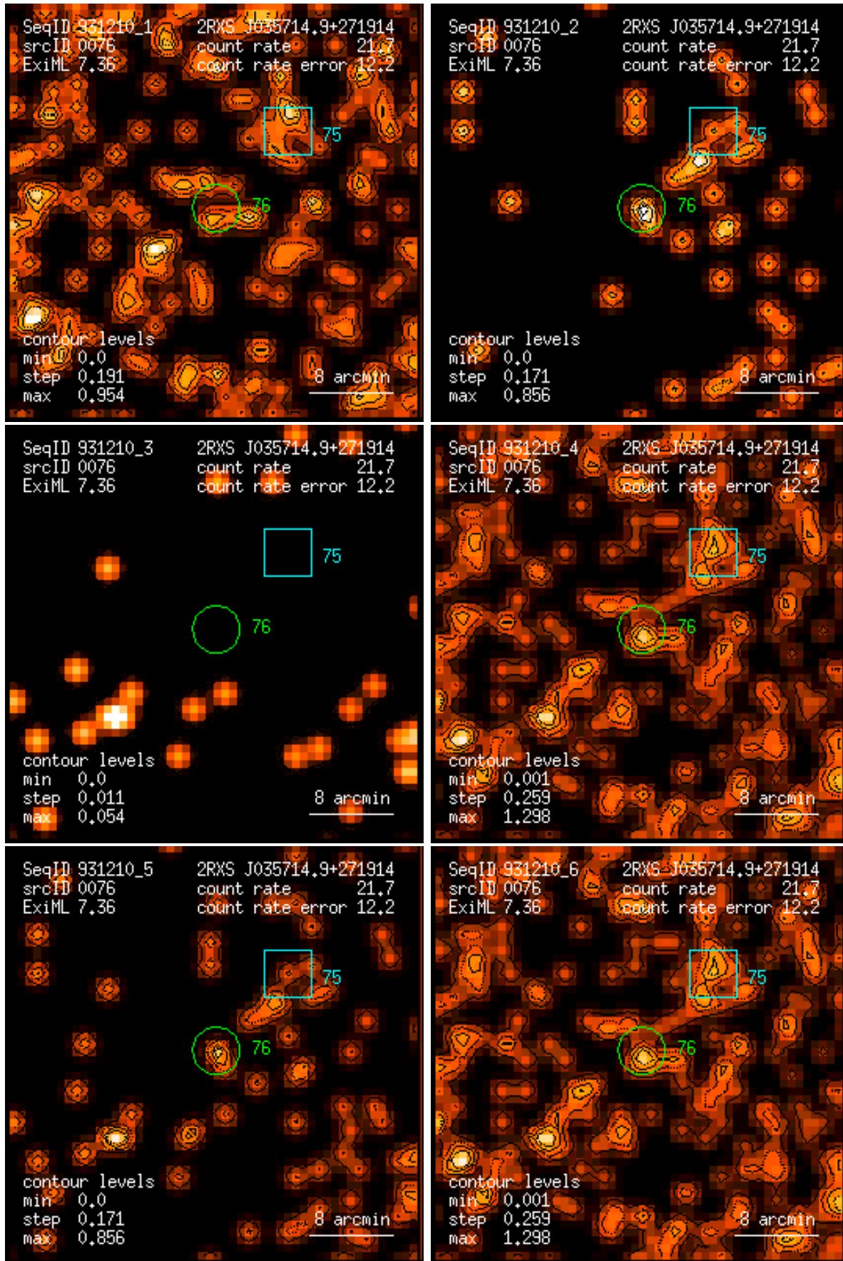
Figure 76: RASS 931210: detection 0076: band rate images, Gaussian filter: (1) PSPC channels 11 – 41, (2) 52 – 90, (3) 91 – 201, (4) 11 – 235, (5) 52 – 201, (6) 11 – 201. Broad band rates in counts/ks. Band rate contour levels in counts/ks/arcmin 2 .
