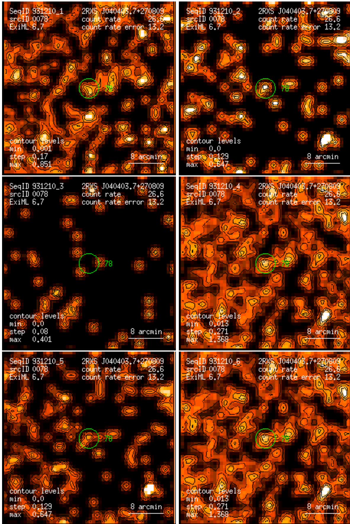
Figure 78: RASS 931210: detection 0078: band rate images, Gaussian filter: (1) PSPC channels 11 – 41, (2) 52 – 90, (3) 91 – 201, (4) 11 – 235, (5) 52 – 201, (6) 11 – 201. Broad band rates in counts/ks. Band rate contour levels in counts/ks/arcmin 2 .
