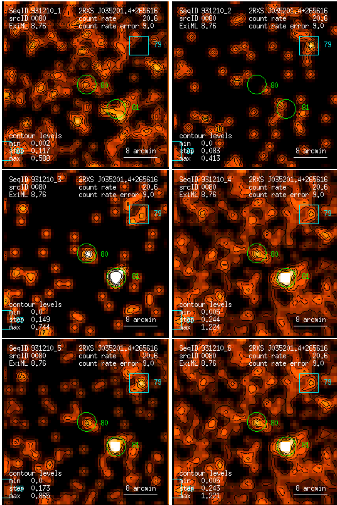
Figure 80: RASS 931210: detection 0080: band rate images, Gaussian filter: (1) PSPC channels 11 – 41, (2) 52 – 90, (3) 91 – 201, (4) 11 – 235, (5) 52 – 201, (6) 11 – 201. Broad band rates in counts/ks. Band rate contour levels in counts/ks/arcmin 2 .
