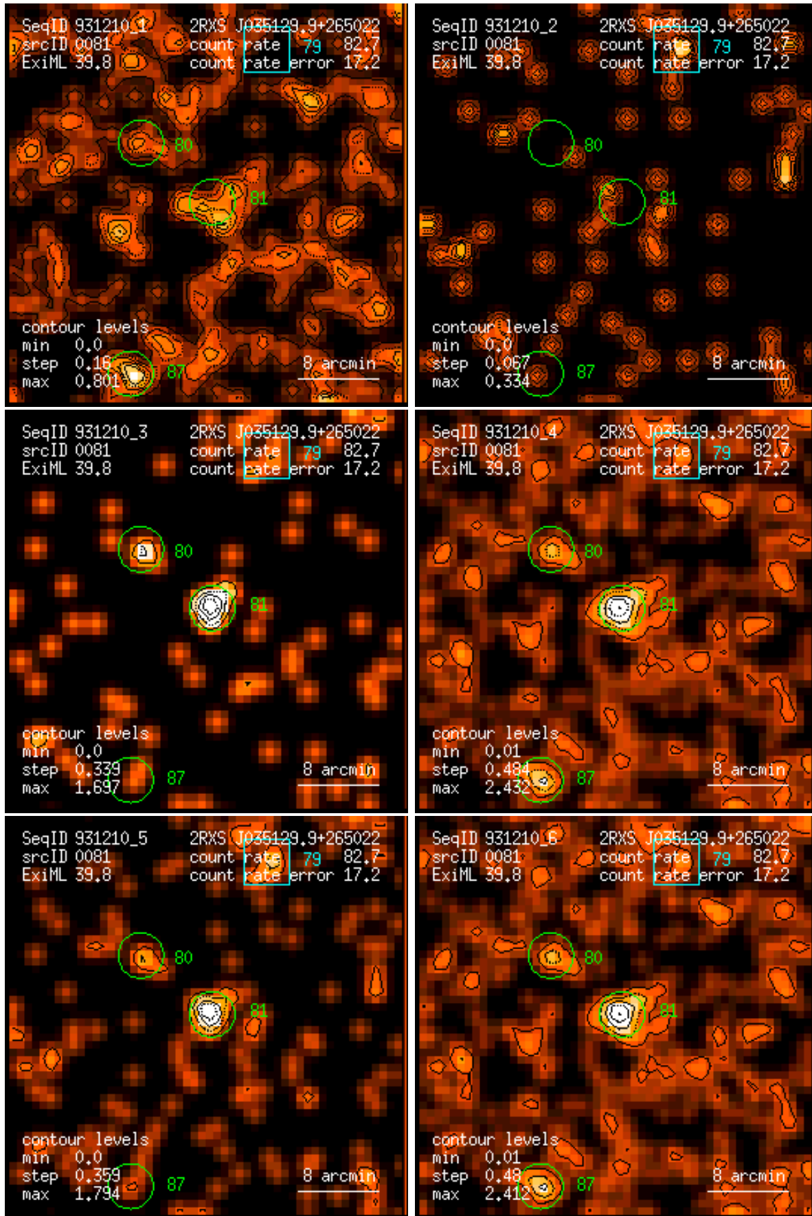
Figure 81: RASS 931210: detection 0081: band rate images, Gaussian filter: (1) PSPC channels 11 – 41, (2) 52 – 90, (3) 91 – 201, (4) 11 – 235, (5) 52 – 201, (6) 11 – 201. Broad band rates in counts/ks. Band rate contour levels in counts/ks/arcmin 2 .
