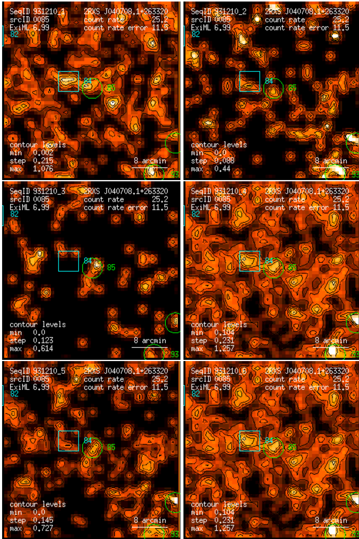
Figure 85: RASS 931210: detection 0085: band rate images, Gaussian filter: (1) PSPC channels 11 – 41, (2) 52 – 90, (3) 91 – 201, (4) 11 – 235, (5) 52 – 201, (6) 11 – 201. Broad band rates in counts/ks. Band rate contour levels in counts/ks/arcmin 2 .
