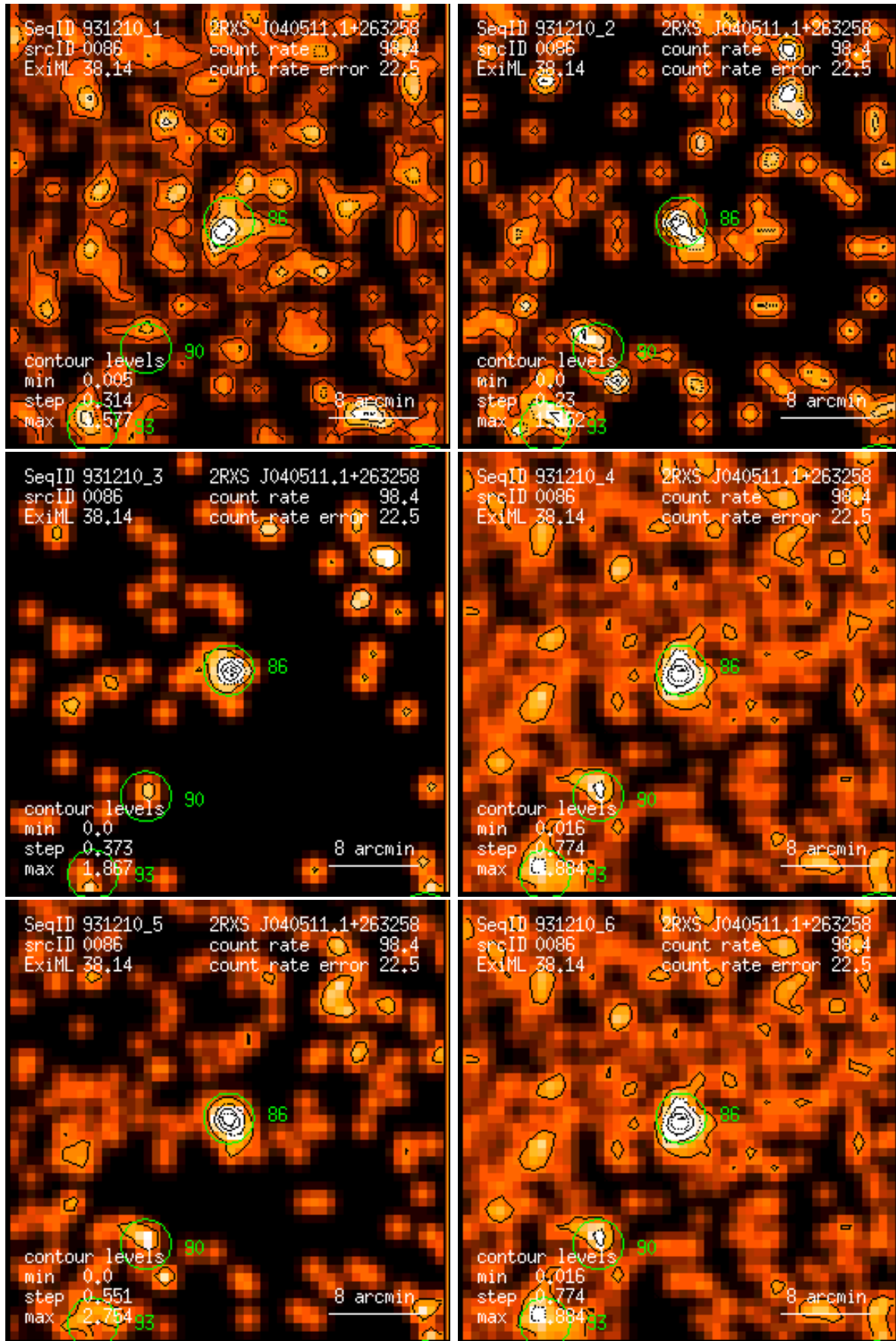
Figure 86: RASS 931210: detection 0086: band rate images, Gaussian filter: (1) PSPC channels 11 – 41, (2) 52 – 90, (3) 91 – 201, (4) 11 – 235, (5) 52 – 201, (6) 11 – 201. Broad band rates in counts/ks. Band rate contour levels in counts/ks/arcmin 2 .
