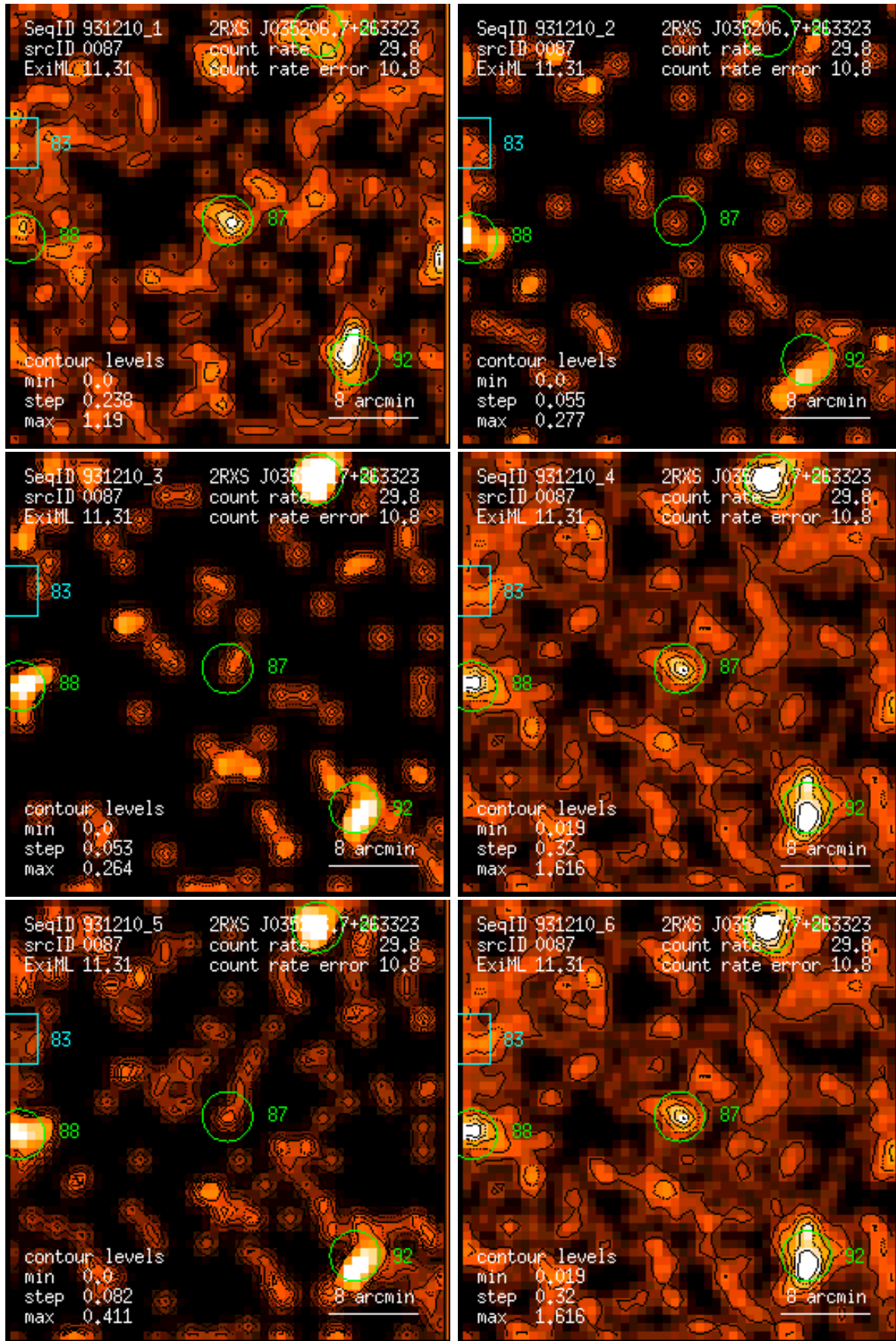
Figure 87: RASS 931210: detection 0087: band rate images, Gaussian filter: (1) PSPC channels 11 – 41, (2) 52 – 90, (3) 91 – 201, (4) 11 – 235, (5) 52 – 201, (6) 11 – 201. Broad band rates in counts/ks. Band rate contour levels in counts/ks/arcmin 2 .
