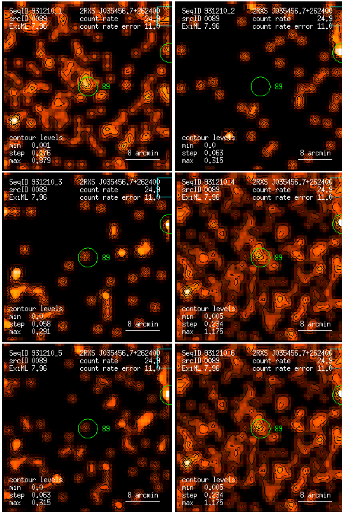
Figure 89: RASS 931210: detection 0089: band rate images, Gaussian filter: (1) PSPC channels 11 – 41, (2) 52 – 90, (3) 91 – 201, (4) 11 – 235, (5) 52 – 201, (6) 11 – 201. Broad band rates in counts/ks. Band rate contour levels in counts/ks/arcmin 2 .
