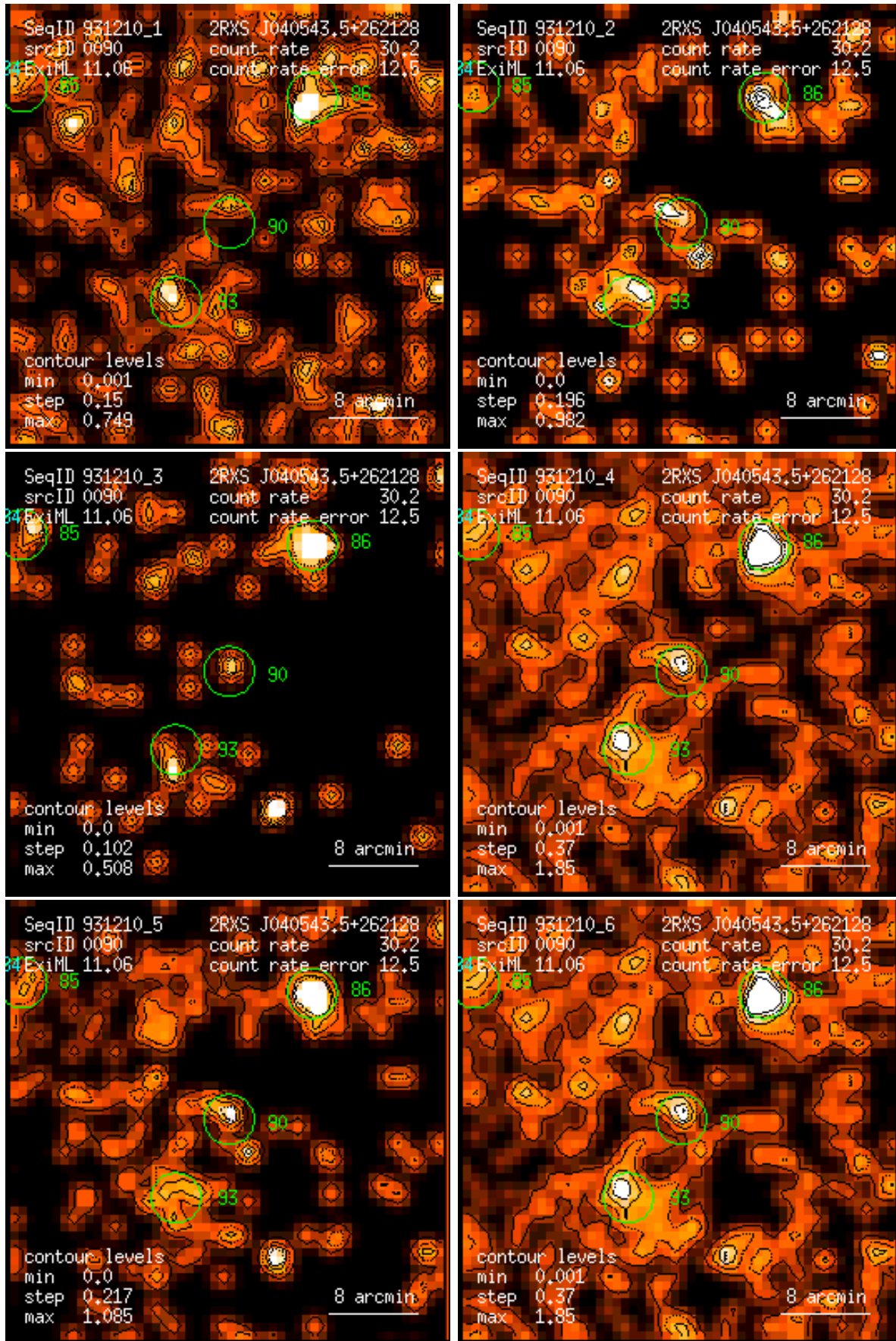
Figure 90: RASS 931210: detection 0090: band rate images, Gaussian filter: (1) PSPC channels 11 – 41, (2) 52 – 90, (3) 91 – 201, (4) 11 – 235, (5) 52 – 201, (6) 11 – 201. Broad band rates in counts/ks. Band rate contour levels in counts/ks/arcmin 2 .
