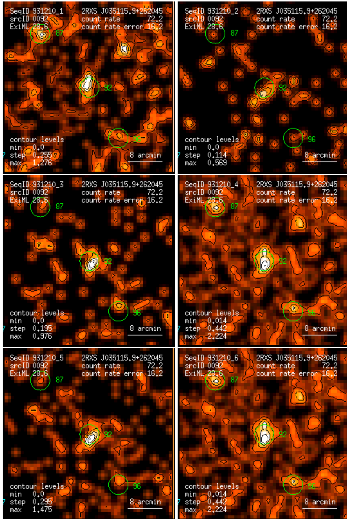
Figure 92: RASS 931210: detection 0092: band rate images, Gaussian filter: (1) PSPC channels 11 – 41, (2) 52 – 90, (3) 91 – 201, (4) 11 – 235, (5) 52 – 201, (6) 11 – 201. Broad band rates in counts/ks. Band rate contour levels in counts/ks/arcmin 2 .
