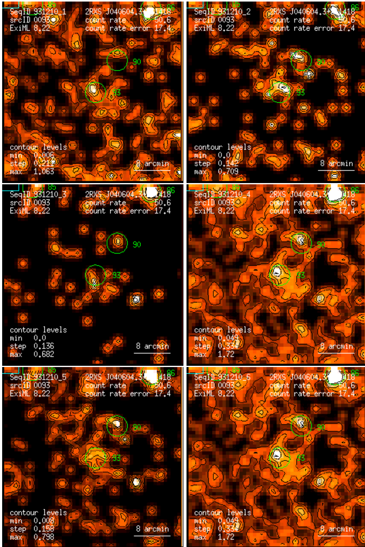
Figure 93: RASS 931210: detection 0093: band rate images, Gaussian filter: (1) PSPC channels 11 – 41, (2) 52 – 90, (3) 91 – 201, (4) 11 – 235, (5) 52 – 201, (6) 11 – 201. Broad band rates in counts/ks. Band rate contour levels in counts/ks/arcmin 2 .
