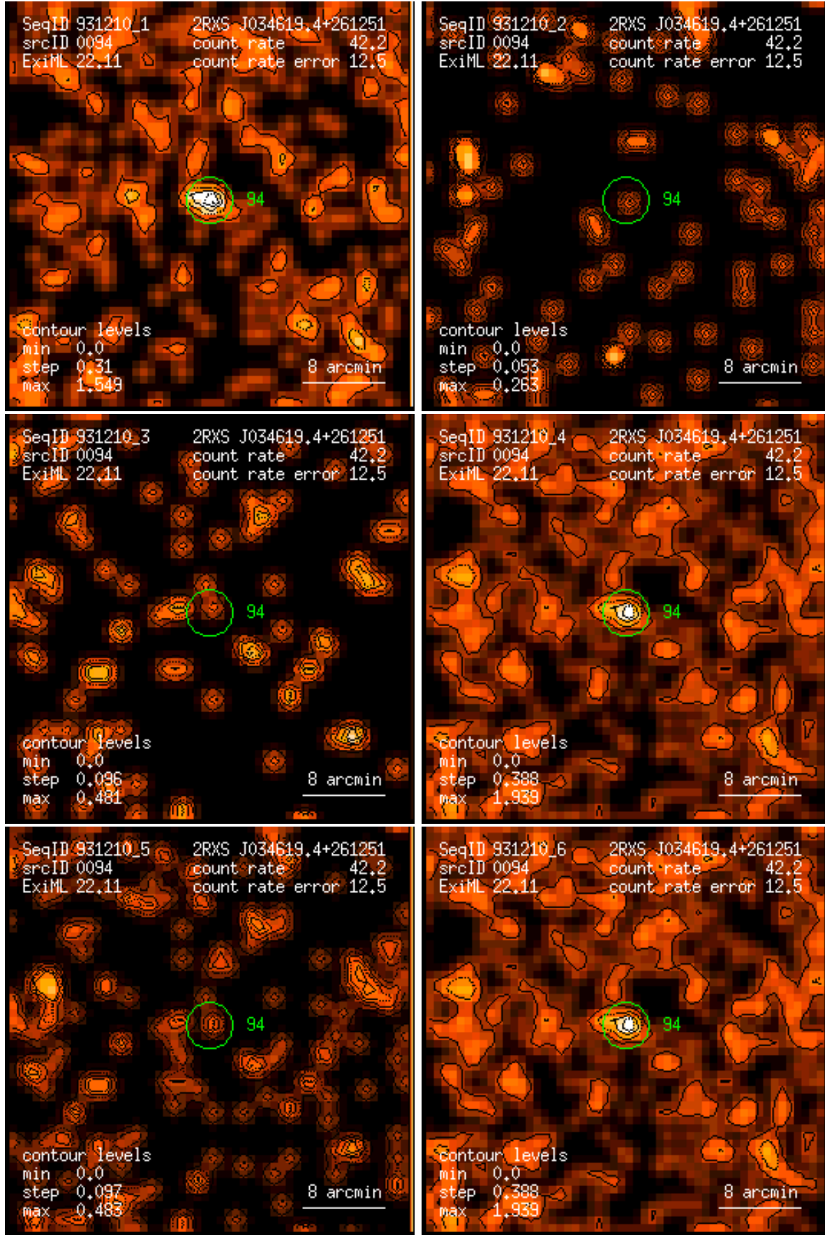
Figure 94: RASS 931210: detection 0094: band rate images, Gaussian filter: (1) PSPC channels 11 – 41, (2) 52 – 90, (3) 91 – 201, (4) 11 – 235, (5) 52 – 201, (6) 11 – 201. Broad band rates in counts/ks. Band rate contour levels in counts/ks/arcmin 2 .
