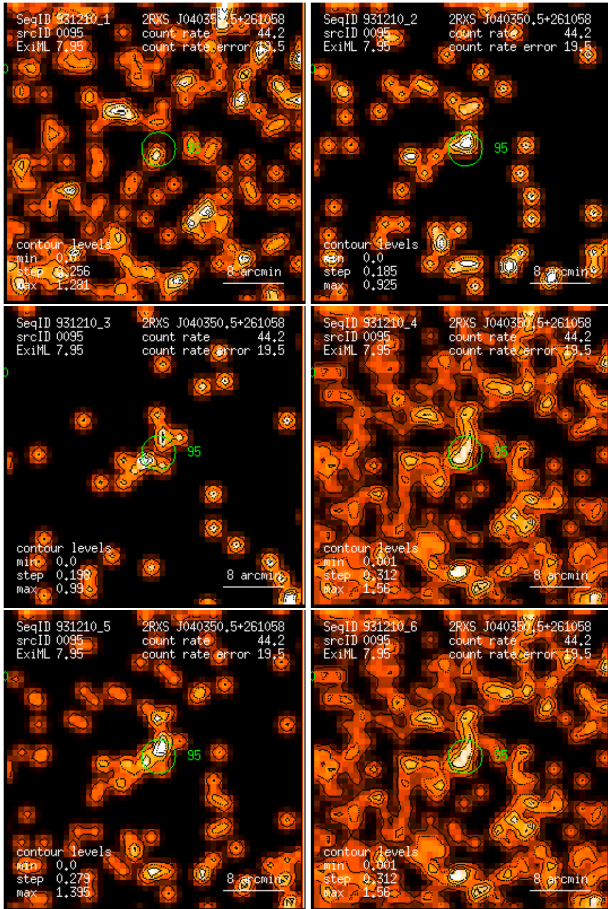
Figure 95: RASS 931210: detection 0095: band rate images, Gaussian filter: (1) PSPC channels 11 – 41, (2) 52 – 90, (3) 91 – 201, (4) 11 – 235, (5) 52 – 201, (6) 11 – 201. Broad band rates in counts/ks. Band rate contour levels in counts/ks/arcmin 2 .
