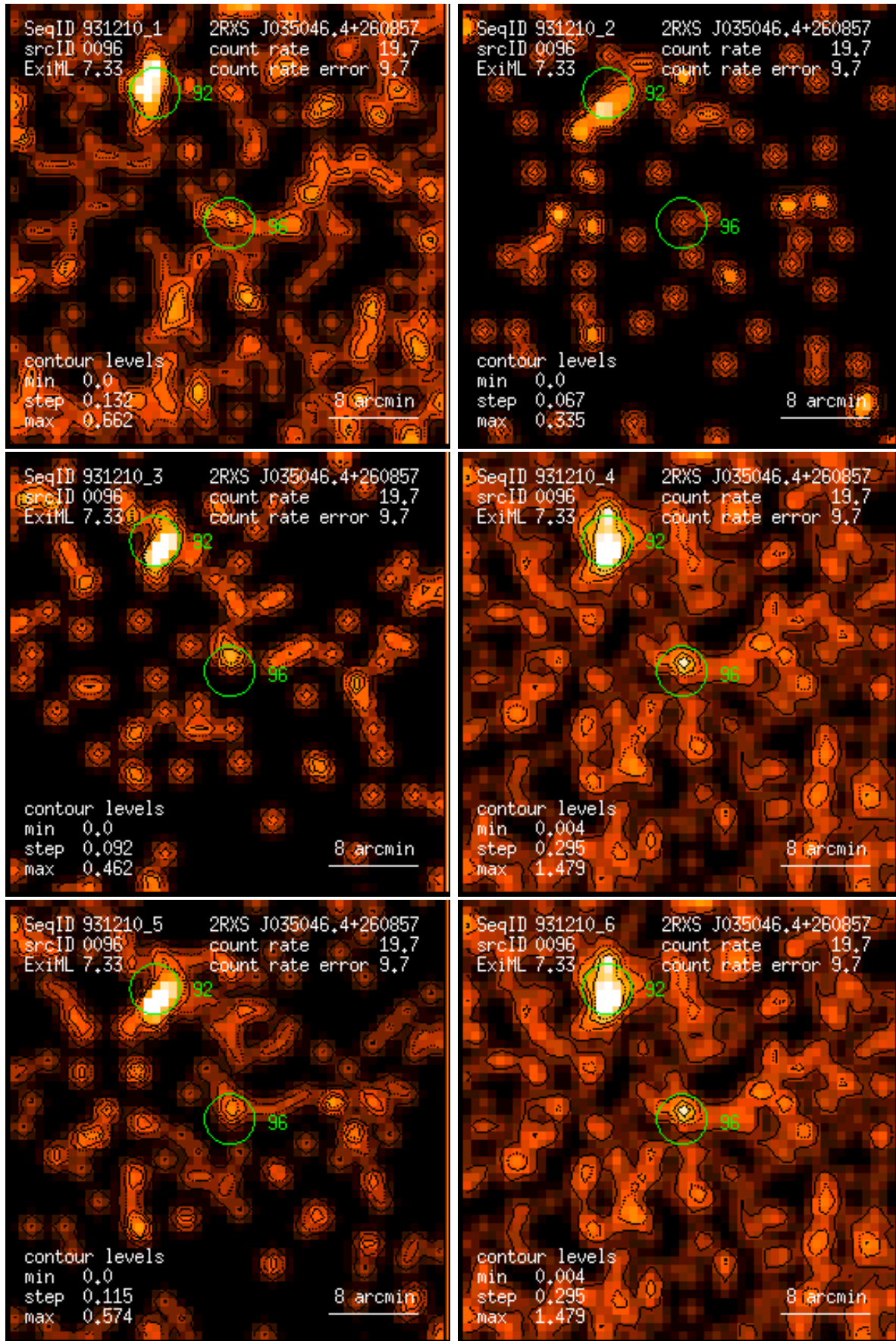
Figure 96: RASS 931210: detection 0096: band rate images, Gaussian filter: (1) PSPC channels 11 – 41, (2) 52 – 90, (3) 91 – 201, (4) 11 – 235, (5) 52 – 201, (6) 11 – 201. Broad band rates in counts/ks. Band rate contour levels in counts/ks/arcmin 2 .
