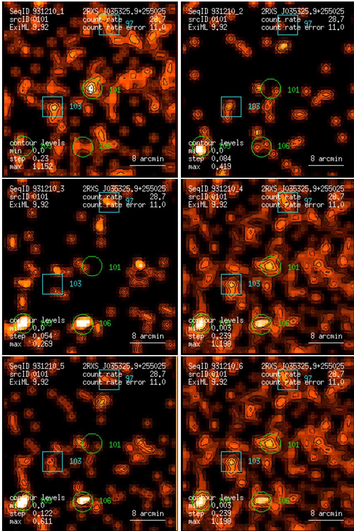
Figure 101: RASS 931210: detection 0101: band rate images, Gaussian filter: (1) PSPC channels 11 – 41, (2) 52 – 90, (3) 91 – 201, (4) 11 – 235, (5) 52 – 201, (6) 11 – 201. Broad band rates in counts/ks. Band rate contour levels in counts/ks/arcmin 2 .
