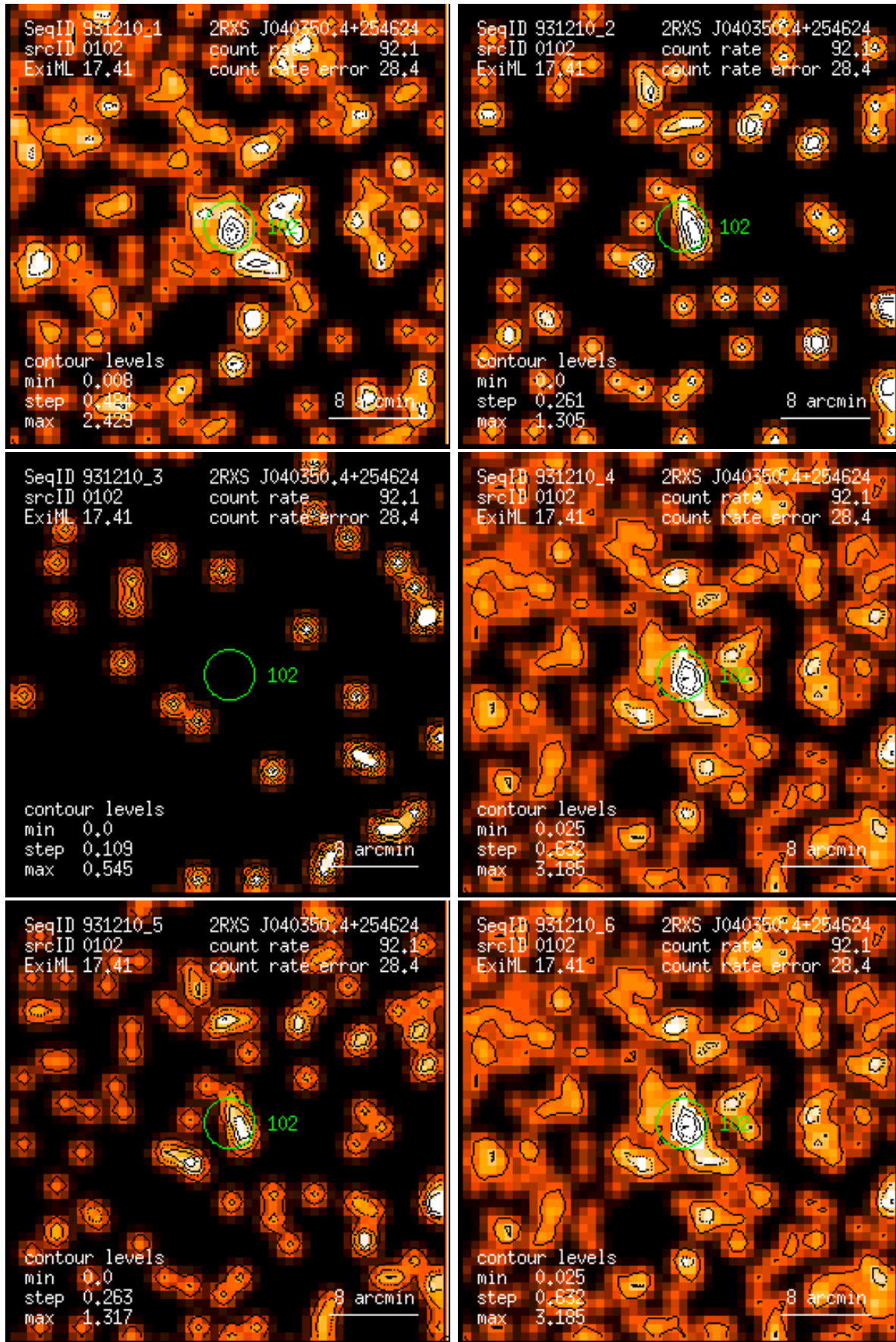
Figure 102: RASS 931210: detection 0102: band rate images, Gaussian filter: (1) PSPC channels 11 – 41, (2) 52 – 90, (3) 91 – 201, (4) 11 – 235, (5) 52 – 201, (6) 11 – 201. Broad band rates in counts/ks. Band rate contour levels in counts/ks/arcmin 2 .
