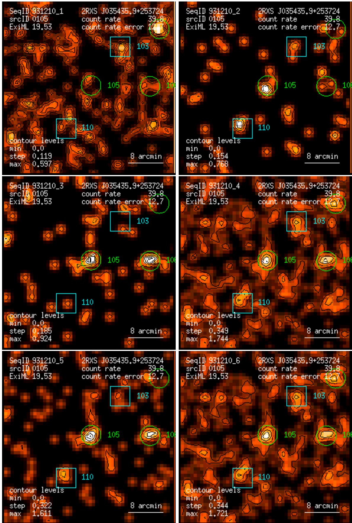
Figure 105: RASS 931210: detection 0105: band rate images, Gaussian filter: (1) PSPC channels 11 – 41, (2) 52 – 90, (3) 91 – 201, (4) 11 – 235, (5) 52 – 201, (6) 11 – 201. Broad band rates in counts/ks. Band rate contour levels in counts/ks/arcmin 2 .
