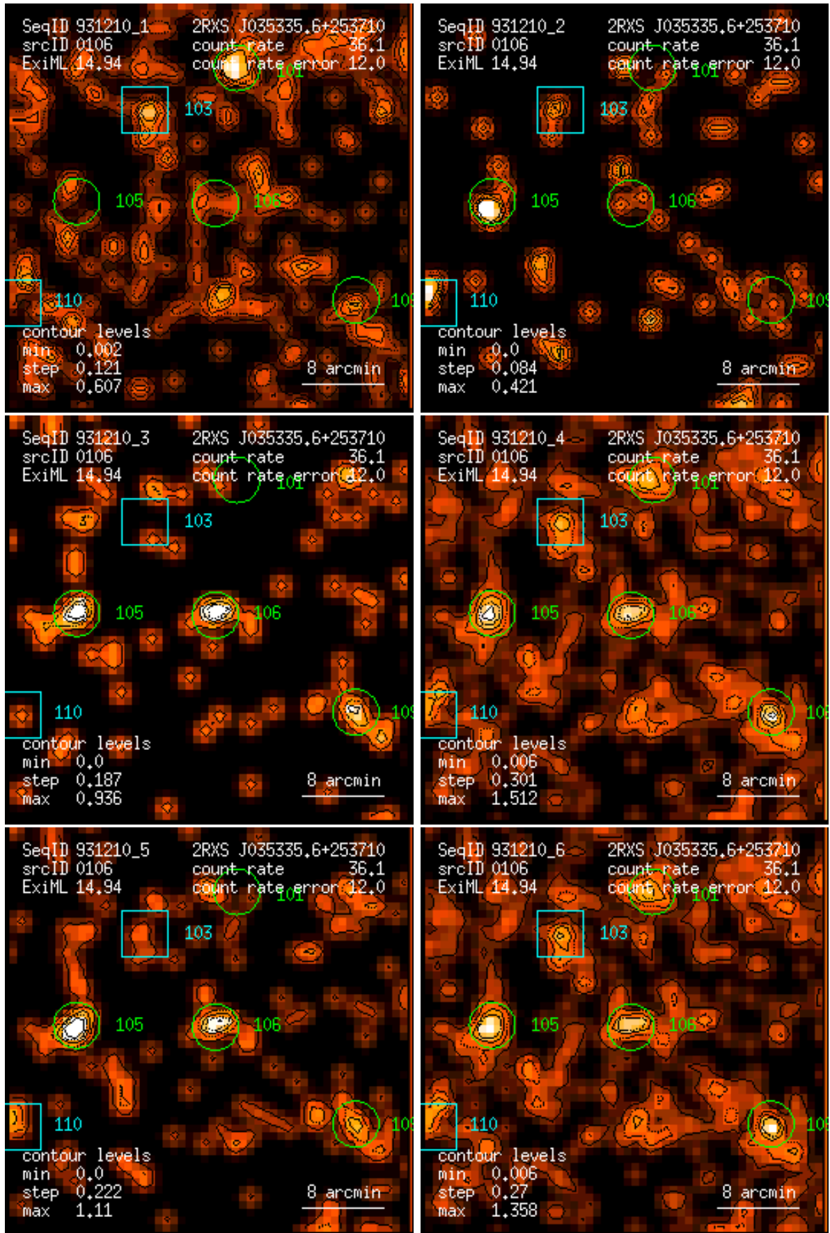
Figure 106: RASS 931210: detection 0106: band rate images, Gaussian filter: (1) PSPC channels 11 – 41, (2) 52 – 90, (3) 91 – 201, (4) 11 – 235, (5) 52 – 201, (6) 11 – 201. Broad band rates in counts/ks. Band rate contour levels in counts/ks/arcmin 2 .
