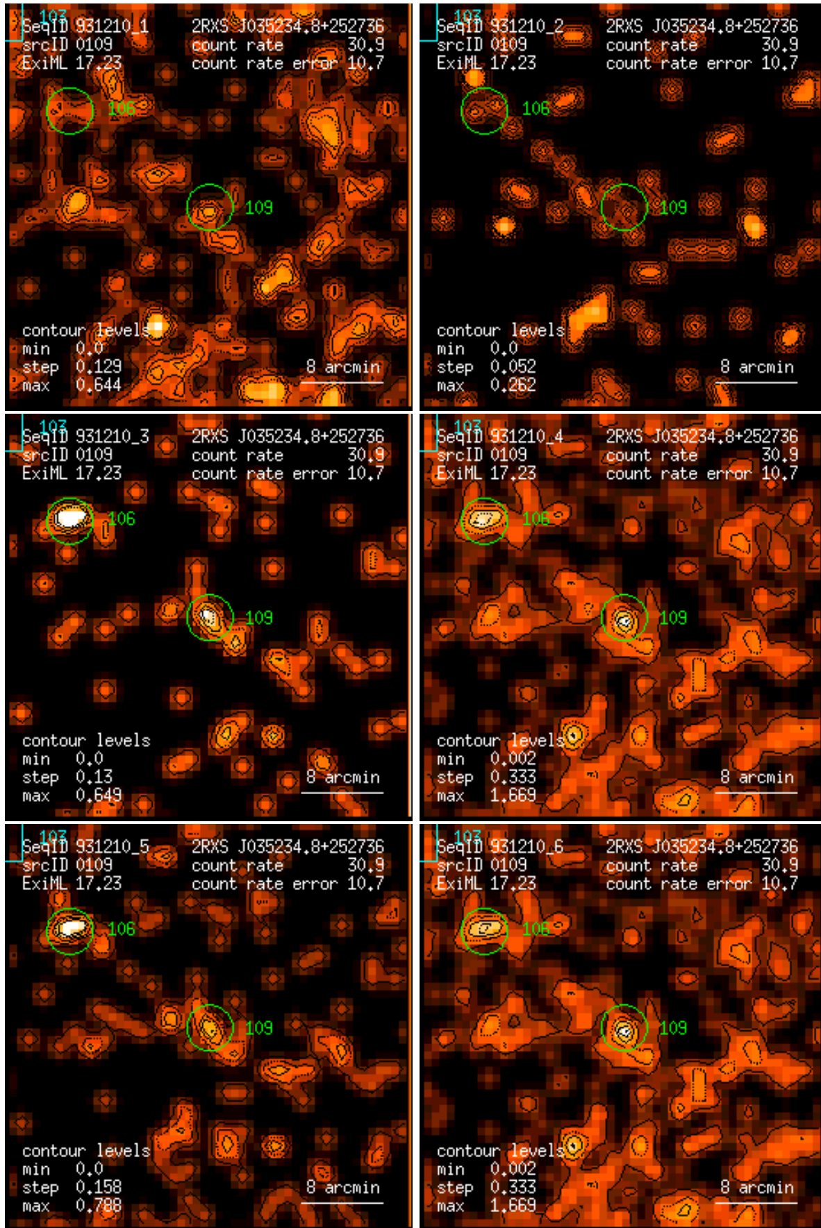
Figure 109: RASS 931210: detection 0109: band rate images, Gaussian filter: (1) PSPC channels 11 – 41, (2) 52 – 90, (3) 91 – 201, (4) 11 – 235, (5) 52 – 201, (6) 11 – 201. Broad band rates in counts/ks. Band rate contour levels in counts/ks/arcmin 2 .
