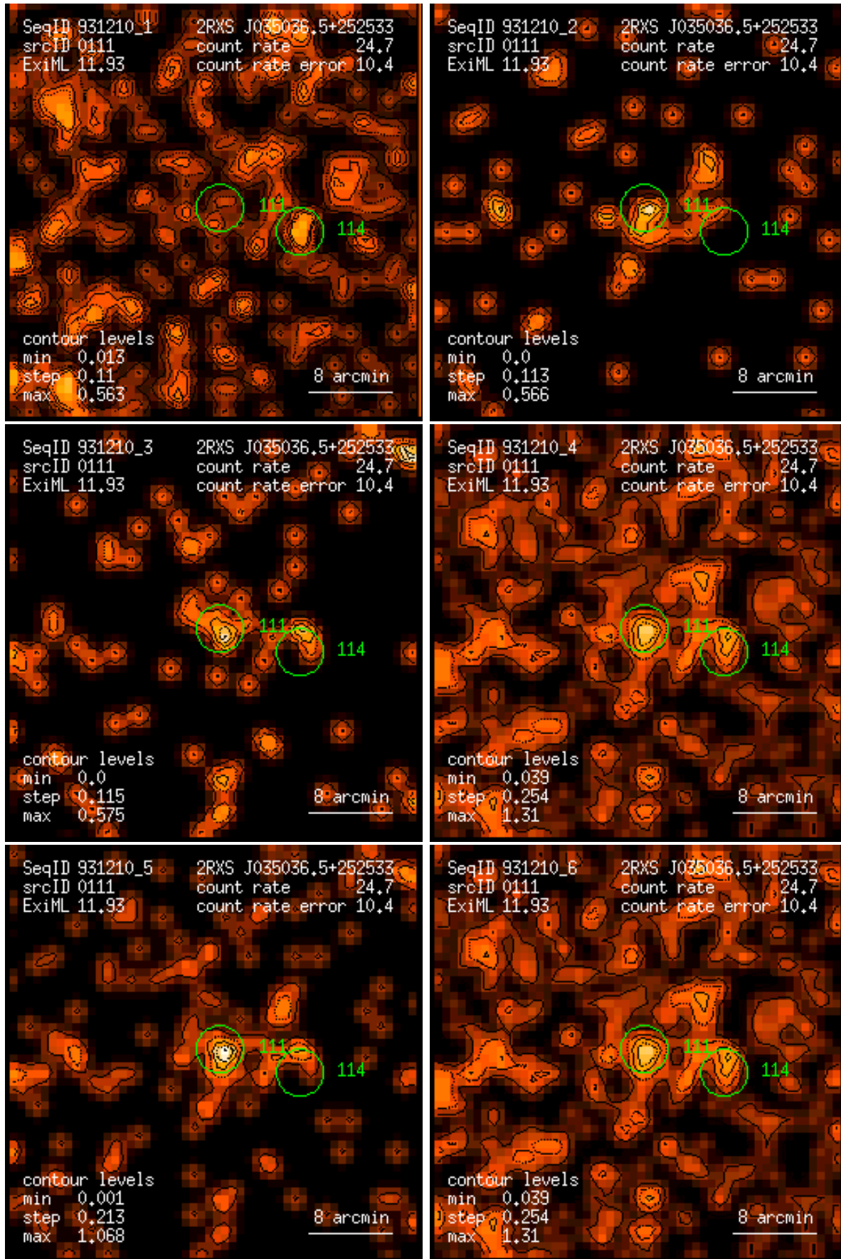
Figure 111: RASS 931210: detection 0111: band rate images, Gaussian filter: (1) PSPC channels 11 – 41, (2) 52 – 90, (3) 91 – 201, (4) 11 – 235, (5) 52 – 201, (6) 11 – 201. Broad band rates in counts/ks. Band rate contour levels in counts/ks/arcmin 2 .
