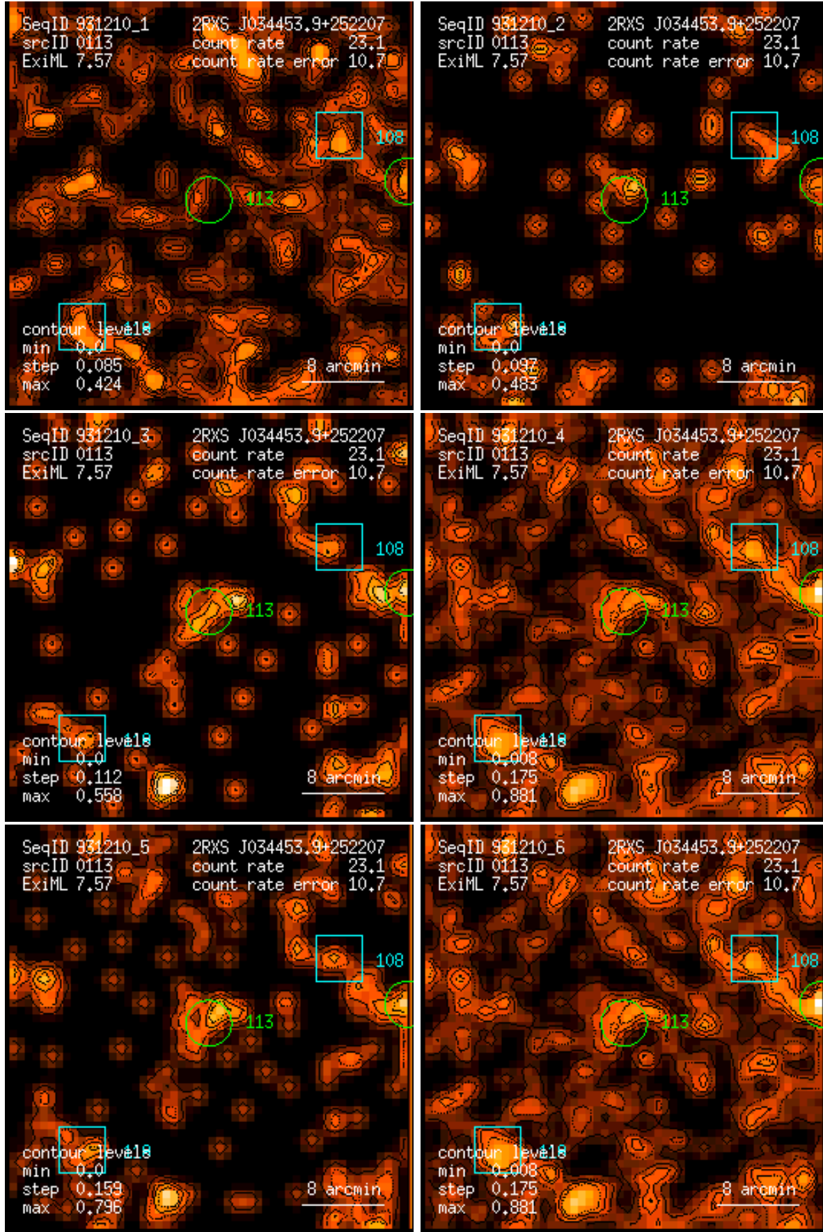
Figure 113: RASS 931210: detection 0113: band rate images, Gaussian filter: (1) PSPC channels 11 – 41, (2) 52 – 90, (3) 91 – 201, (4) 11 – 235, (5) 52 – 201, (6) 11 – 201. Broad band rates in counts/ks. Band rate contour levels in counts/ks/arcmin 2 .
